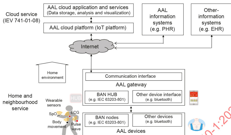
Figure 9 – Example of a BAN system (cloud computing outside the home environment, e.g., in the neighbourhood)
