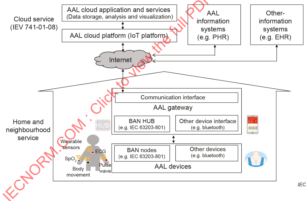
Figure 8 – Example of a BAN system (cloud computing at home)
