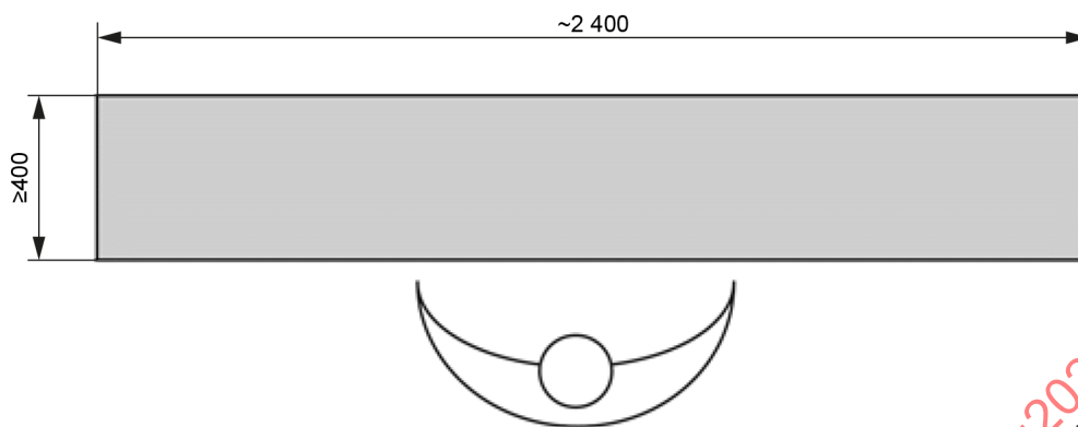
Figure 101 – Test set-up for cut-off machines
