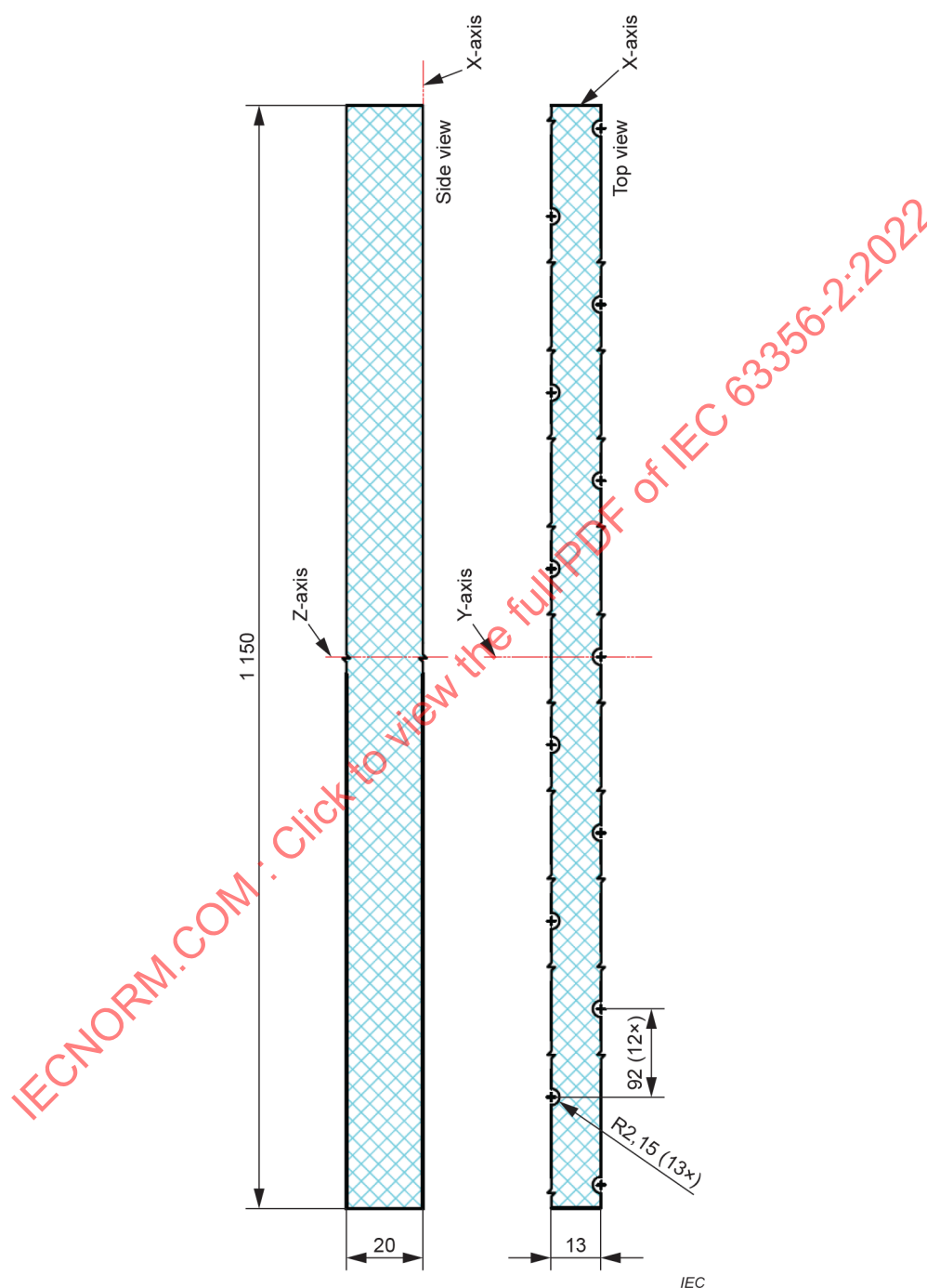
Figure 19 – LED module demarcation of the L115W1 category
