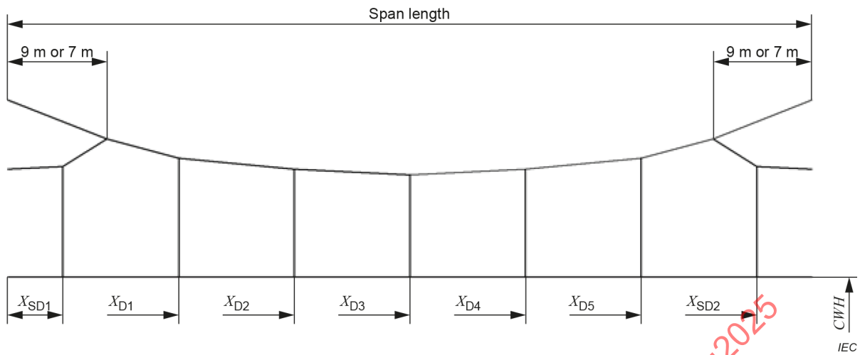
Figure B.2 – Basic dropper arrangement span type ST1
