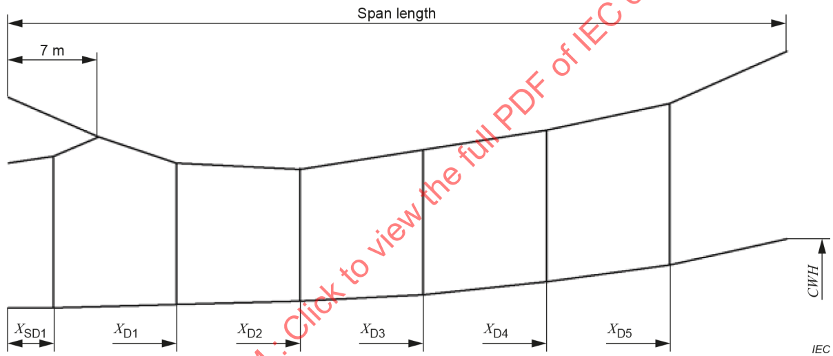
Figure B.3 – Basic dropper arrangement span type ST2
