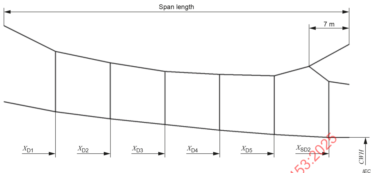
Figure B.8 – Basic dropper arrangement span type ST7
