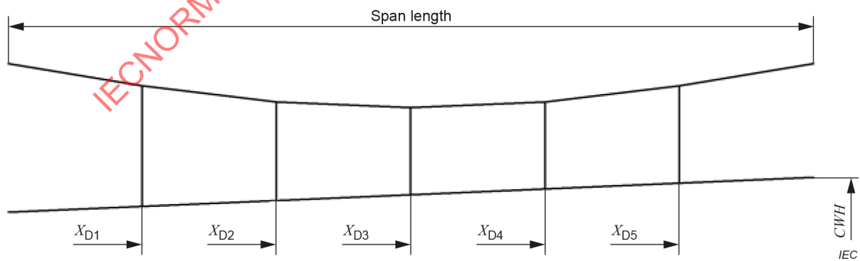
Figure B.4 – Basic dropper arrangement span type ST3
