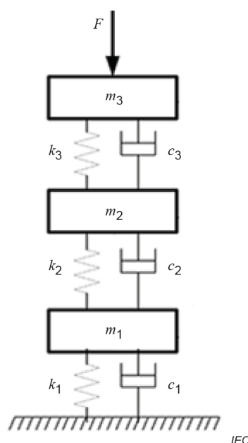
Figure A.4 – Pantograph model
