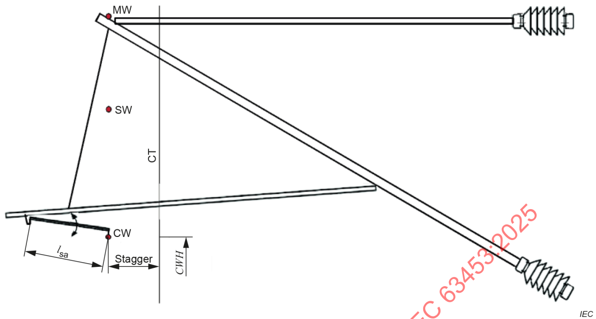
Figure B.10 – Basic support arrangement Mast Type MT2 (push-off)
