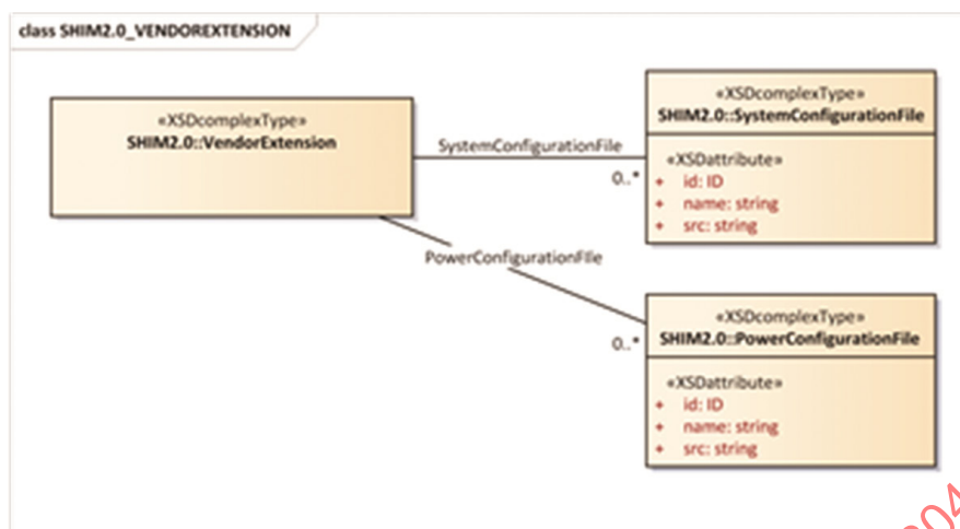
Figure 18—Schema of VendorExtension
