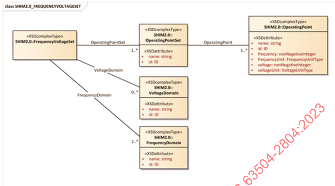
Figure 13—Schema of FrequencyVoltageSet
