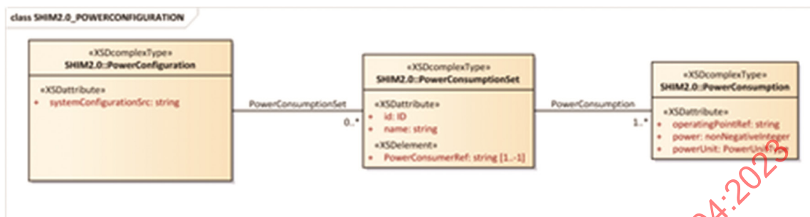
Figure 17—Schema of PowerConfiguration
