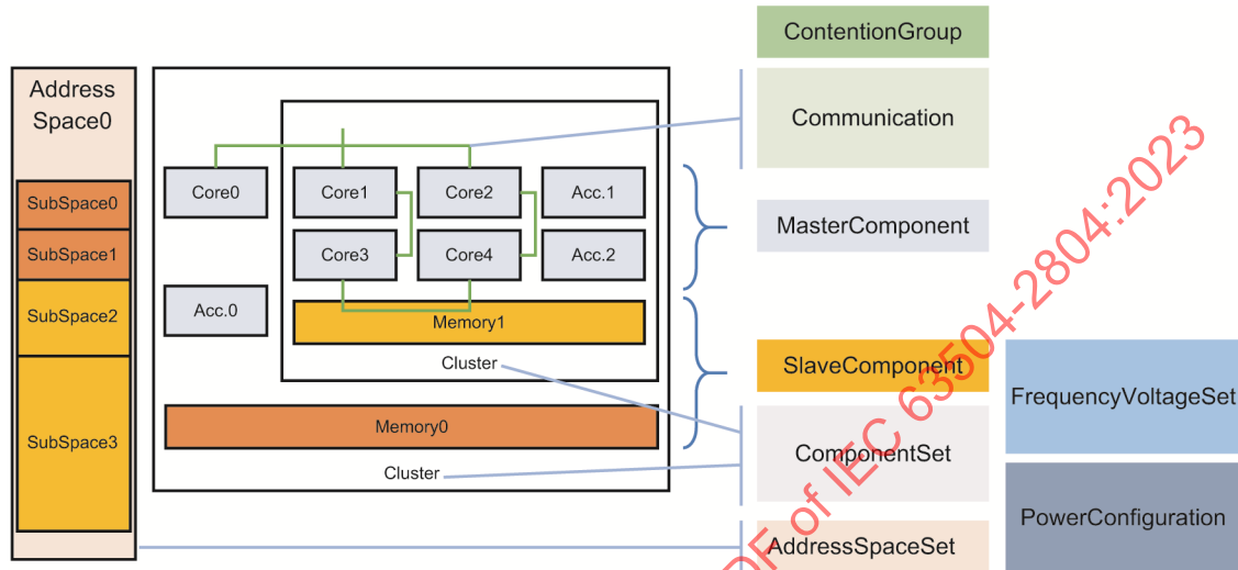
Figure 2—The SHIM elements mapped to a pseudo-multicore hardware
