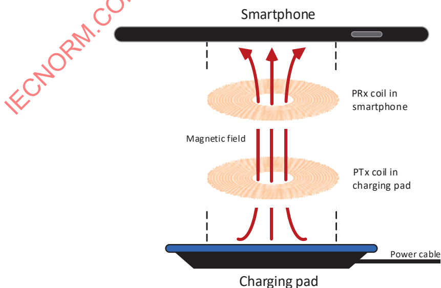
Figure 3. Qi wireless power transfer using magnetic induction
