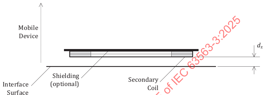
Figure 2. Secondary Coil assembly
