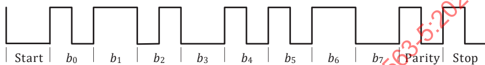
Figure 4. Example of the asynchronous serial format
