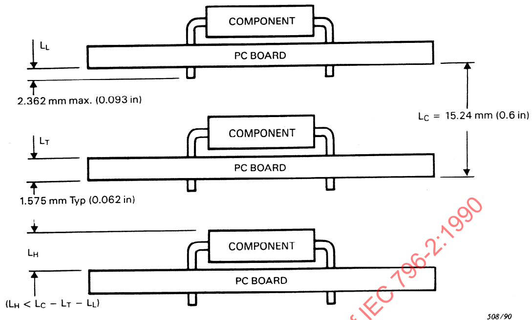
Fig. 1. - Backplane card to card separation.
