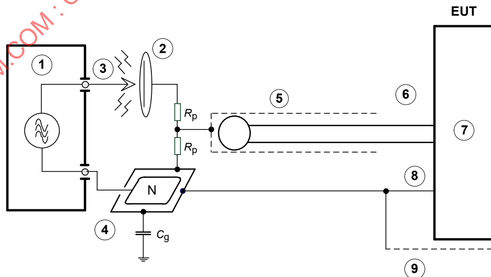
Figure 202.103 – Test setup for HF SURGICAL EQUIPMENT protection measurement according to 202.8.102
