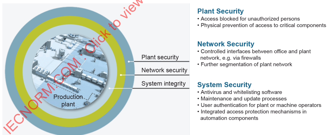
Figure 7 – Selected measures for defence-in-depth strategy
