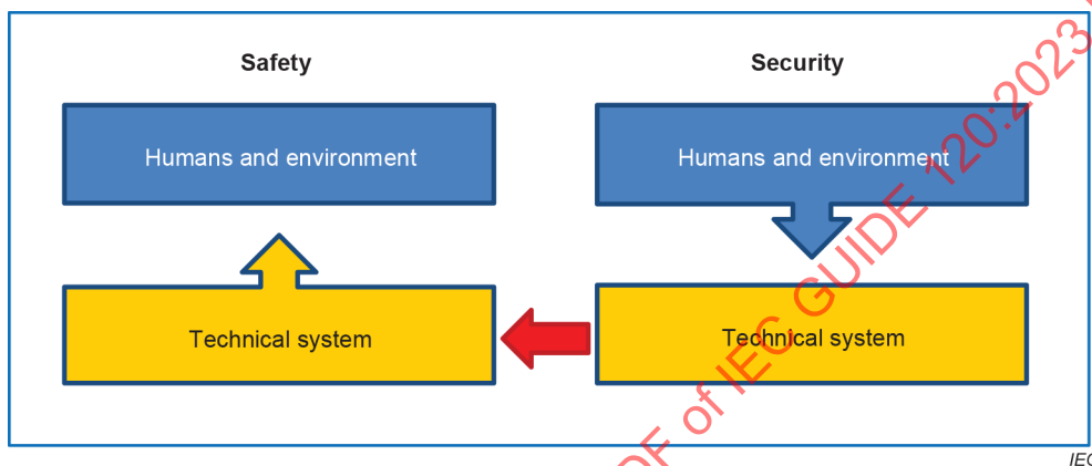
Figure 5 – Interrelation between functional safety and security
