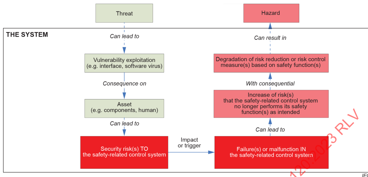
Figure 8 – Possible impact of security risk or risks on the safety-related control system
