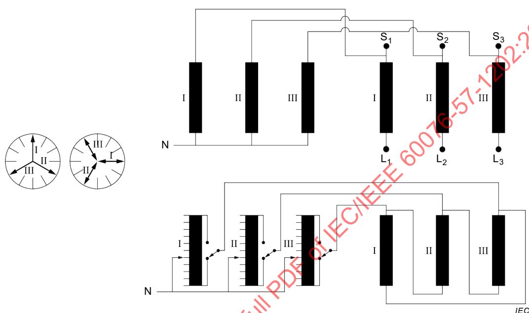
Figure 5 – Exemple E: YNyn+d/IIIId A0-3/9
