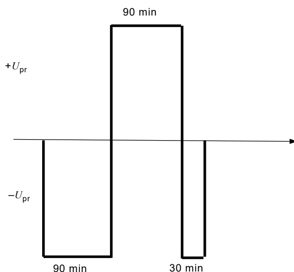
Figure 1 – Double reversal test voltage profile
