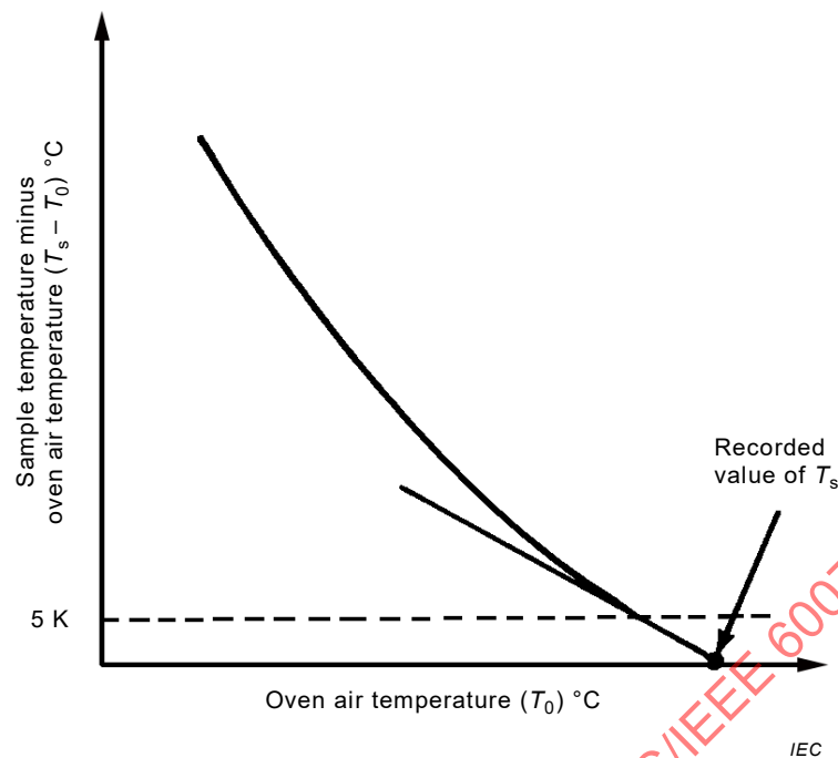
Figure 7 – Maximum sheath temperature using product classification approach
