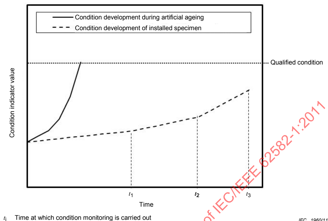
Figure 3 – Illustration of condition-based qualification
