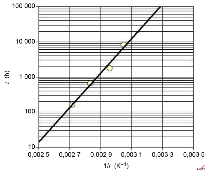
Figure 1 – Example of an Arrhenius diagram
