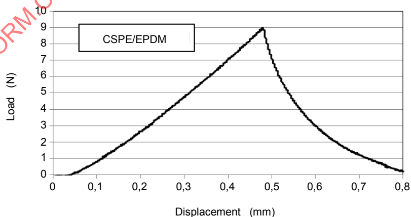
Figure B.1 – Example of measured force vs displacement
