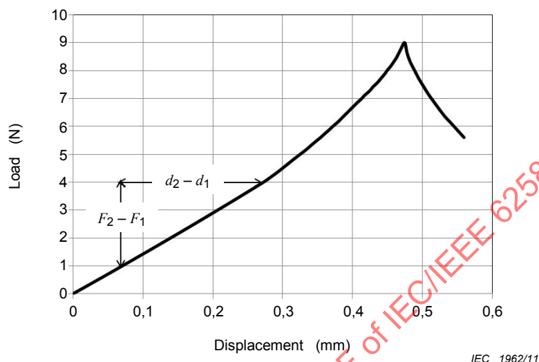
Figure 2 – Calculation of indenter modulus
