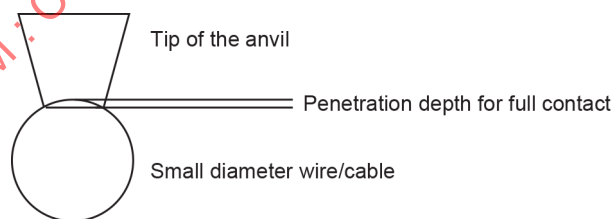
Figure 2 – Penetration depth for full contact on the tip of the anvil
