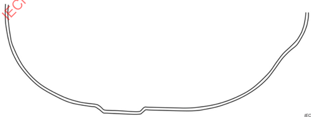
Figure 4 – Cross-sectional view of SAM virtual phantom for PD evaluations at the reference plane (shell thickness is 2 mm everywhere, including at the pinna)
