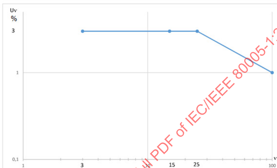
Figure 3 – Single harmonic distortion limits
