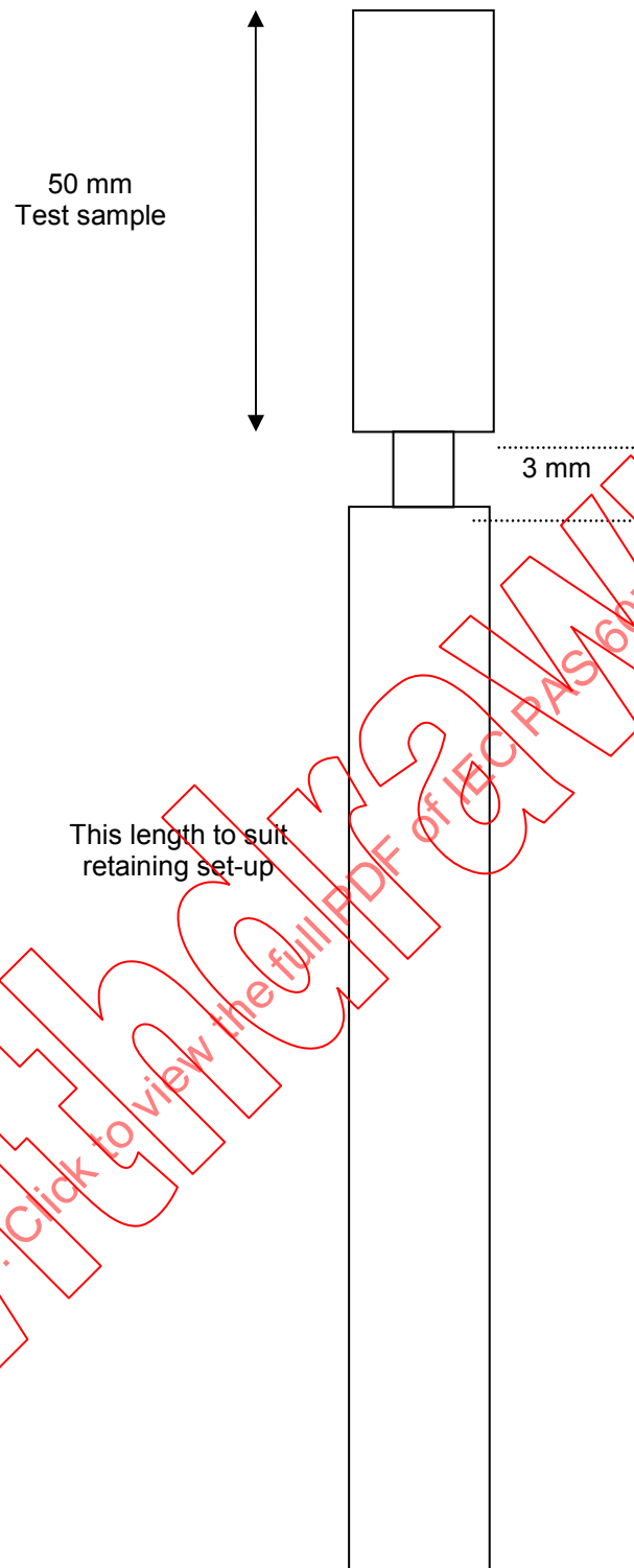
Figure A.3 – Cable sample preparation
