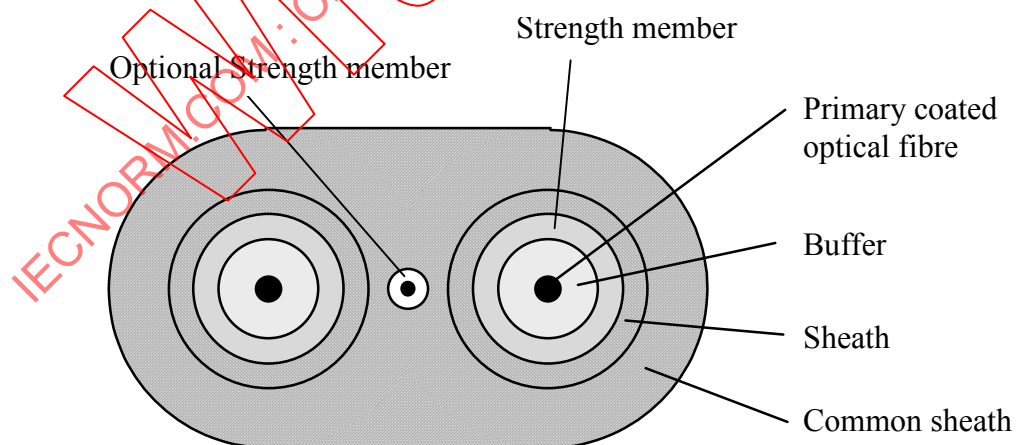
Figure 6 – Duplex flat cable
