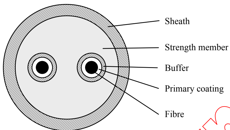
Figure 4 – Duplex ruggedized fibre cable
