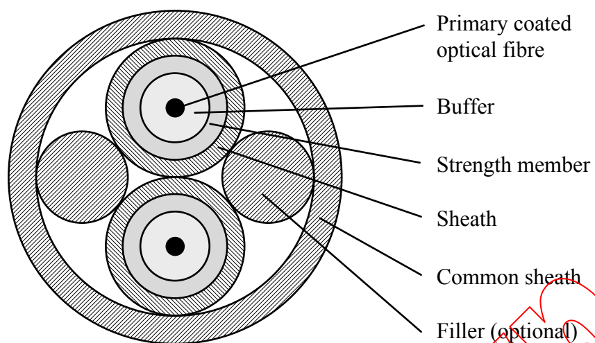
Figure 7 – Duplex round cable
