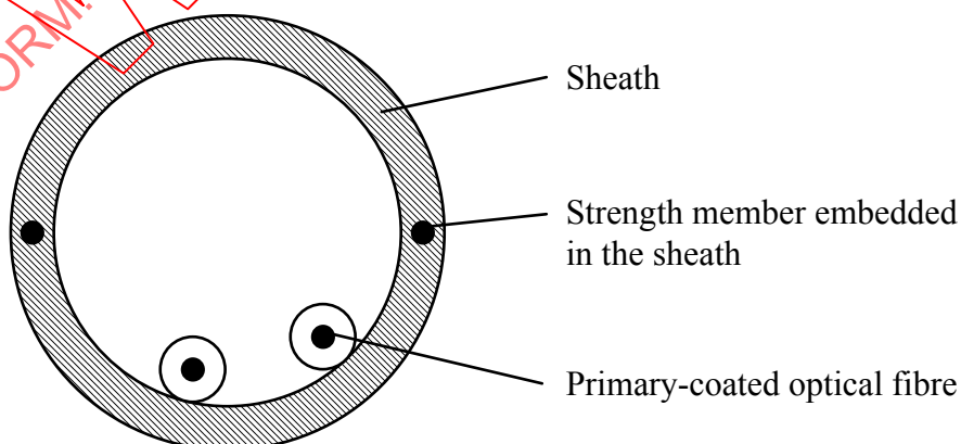
Figure 3 – Duplex loose non-buffered fibre cable
