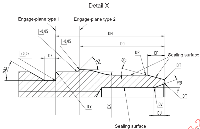
Figure 26 – Outer push-pull locking: female fixed connector side view with details and engage-plane definition for male free cable connector
