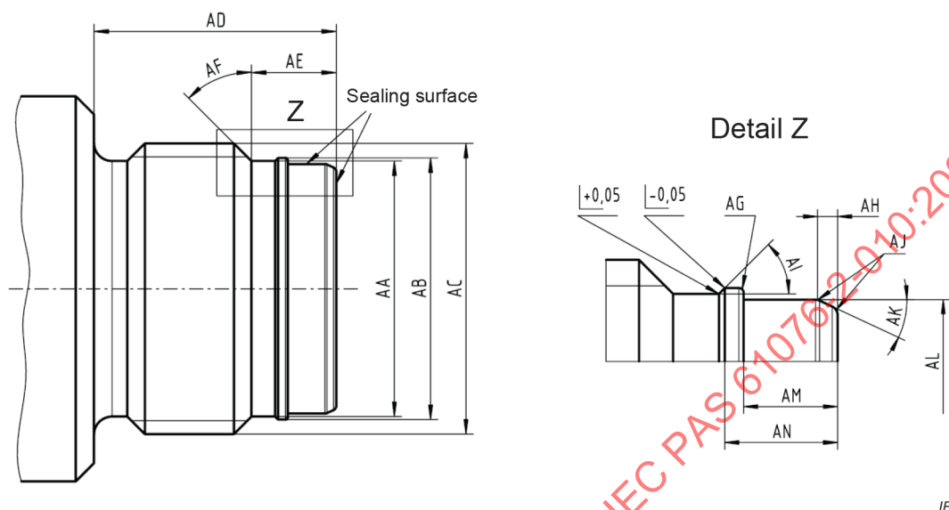
Figure 25 – Outer push-pull locking: male fixed connector side view
