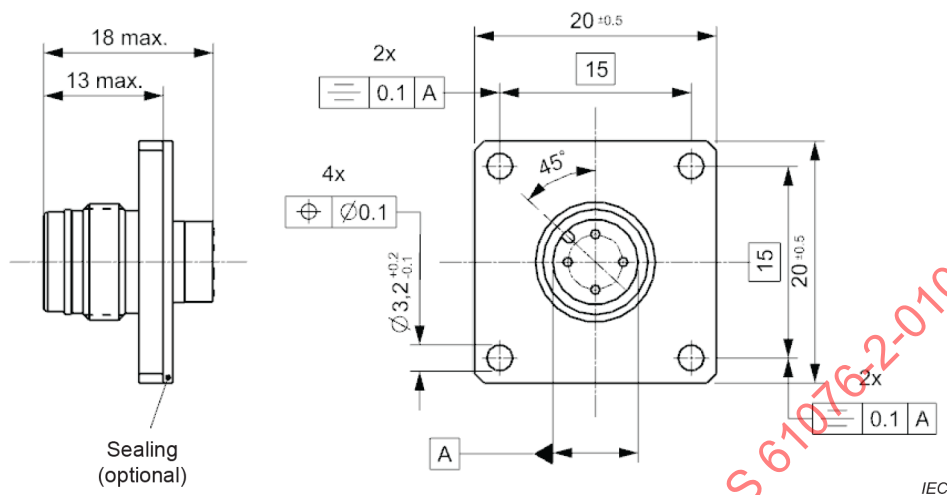
Figure 2 – Fixed connector, male contacts, mounting with thread M12 × 1 and outer push-pull locking, square flange front mounting
