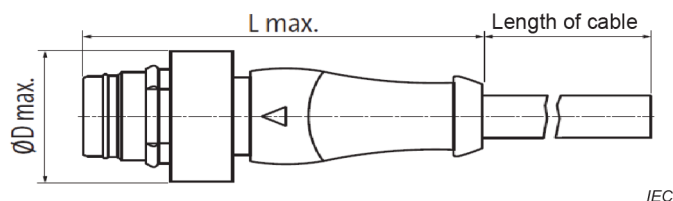
Figure 23 – Non-rewireable connector, male contacts, straight version, with inner push-pull locking
