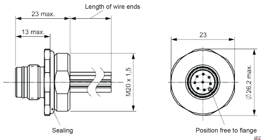
Figure 4 – Fixed connector, male contacts, mounting with thread M12 × 1 and outer push-pull locking, with wire ends, single hole front mounting thread M20 × 1,5
