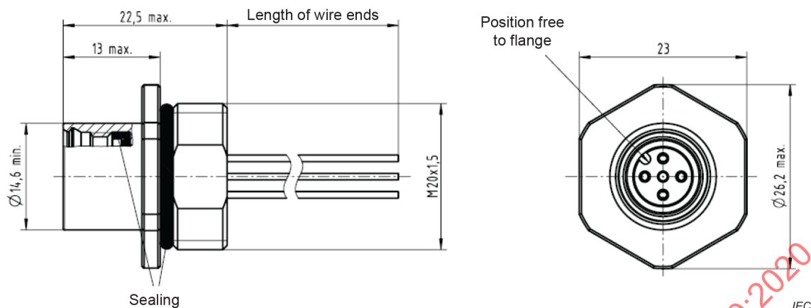
Figure 10 – Fixed connector, female contacts, mounting with thread M12 × 1 and inner push-pull locking, with wire ends, single hole front mounting thread M20 × 1,5
