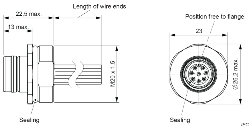
Figure 6 – Fixed connector, female contacts, mounting with thread M12 × 1 and outer push-pull locking, with wire ends, single hole front mounting thread M20 × 1,5
