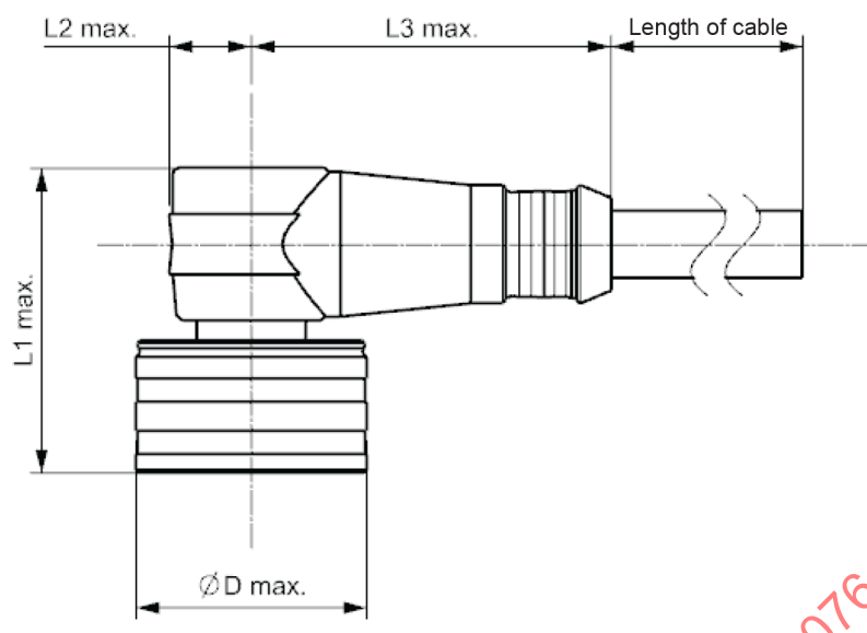
Figure 20 – Non-rewireable connector, female contacts, angled version, with outer push-pull locking
