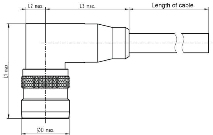
Figure 16 – Non-rewireable connector, male contacts, angled version, with outer push-pull locking
