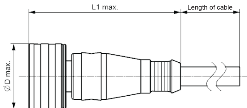
Figure 19 – Non-rewireable connector, female contacts, straight version, with outer push-pull locking
