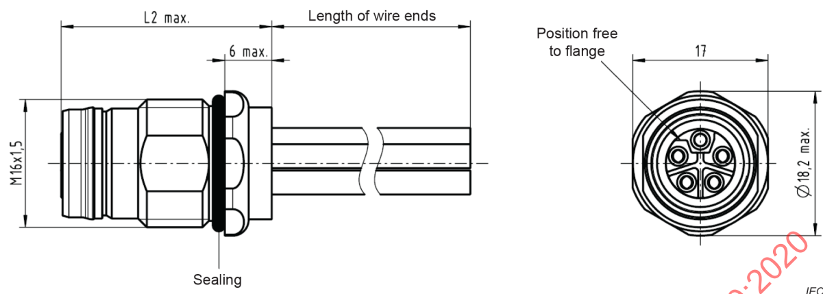
Figure 8 – Fixed connector, female contacts, mounting with thread M12 × 1 and outer push-pull locking, with wire ends, single hole rear mounting thread M16 × 1,5
