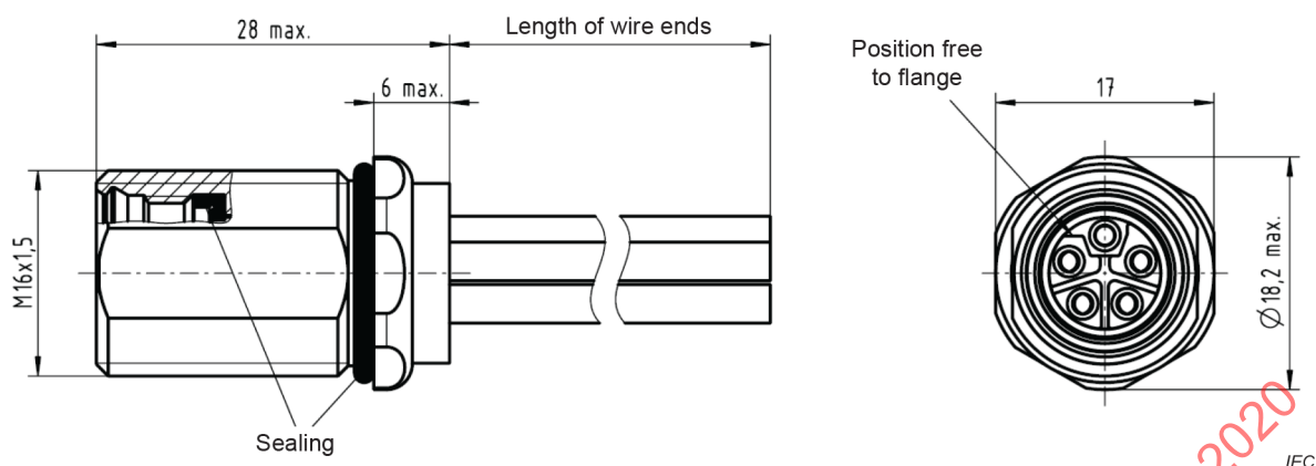
Figure 12 – Fixed connector, female contacts, mounting with thread M12 × 1 and inner push-pull locking, with wire ends, single hole rear mounting thread M16 × 1,5
