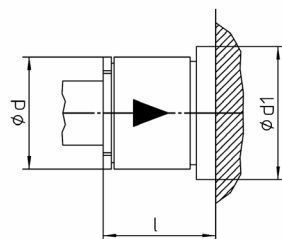
Figure 6a - Housing variant 1
