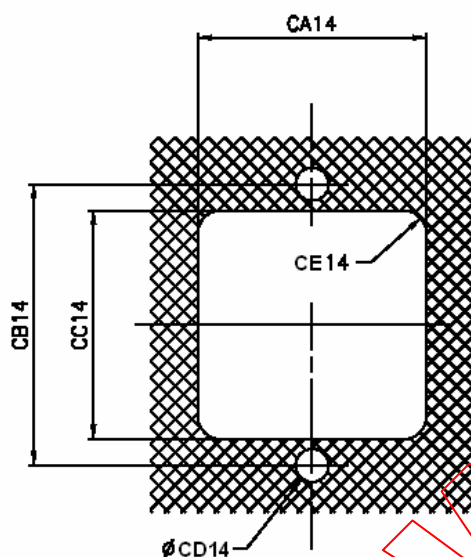
Figure 3 – Variant 13 mounting
