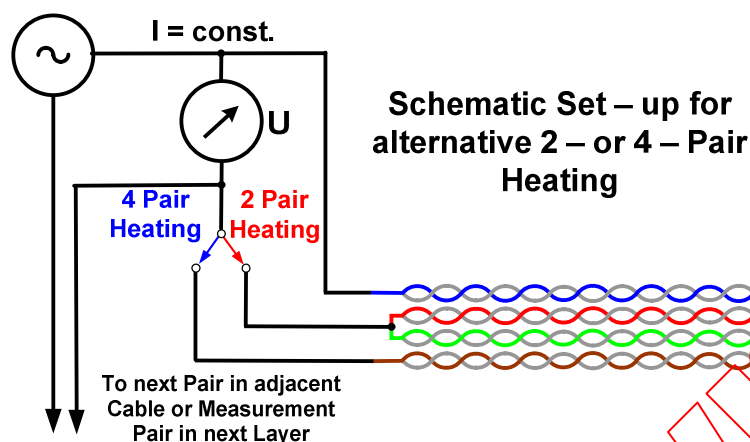
Figure 5 – Connections on both ends of the center cable to obtain two nearly identical “pair” resistances, which can then be measured using the voltage across these pairs
