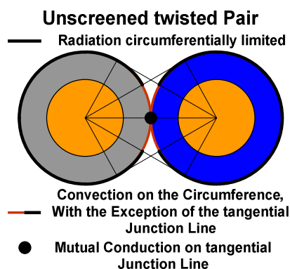
Figure 10 – Dissipation of an unscreened twisted pair exposed to current heating
