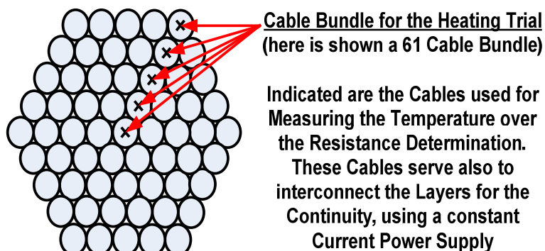
Figure 4 – Cross-section of a cable bundle used for the test, here a bundle of 61 cables
