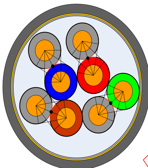
Figure 13 – Heat dissipation of an overall screened cable
