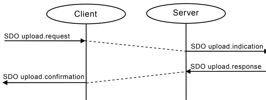
Figure 10 – Successful SDO upload sequence
