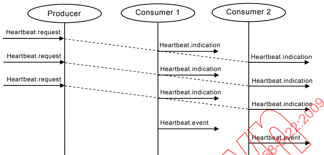
Figure 15 – Heartbeat sequence
