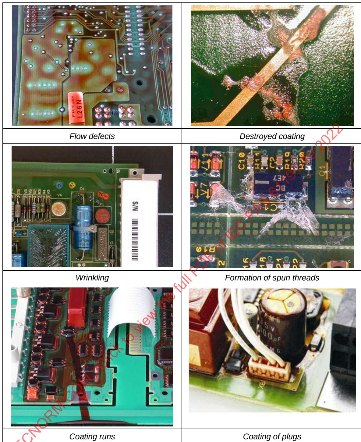
Fig. 12: Examples of typical error patterns
