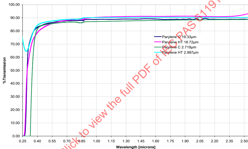
Fig. C17: Transmission spectrum of Parylene C and Parylene HT covering 0.25 \mu to 2.5 \mu
