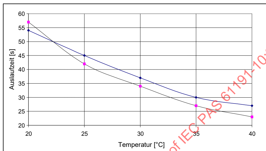
Fig. H3: Viscosity as a function of temperature (4 mm outlet cup, 20°C)
