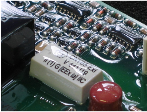
Fig. C22: Examples for a coating with thick-film protective coating
