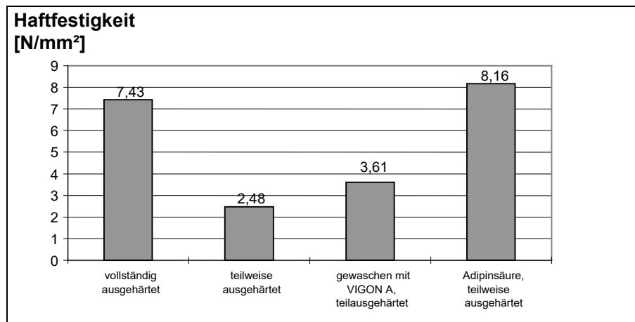
Fig. D9: Influence of surface quality on the adhesion of a PUR protective coating on Sn60Pb
