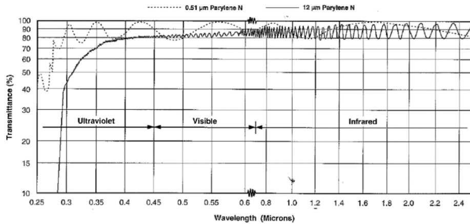
Fig. C16: Transmission spectrum of Parylene N covering 0.25 \mu to 2.4 \mu
