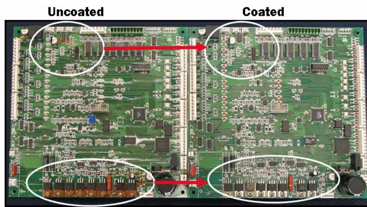
PCB boards with Parylene HT® after 144 hours salt fog test in accordance with ASTM B117-(03)
