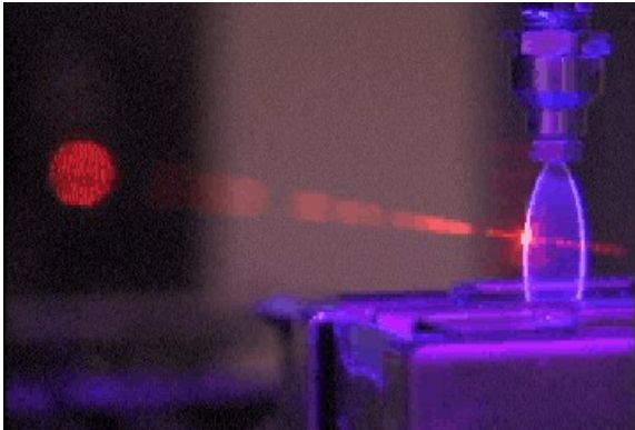
Fig. G16: Automatic monitoring of the fan pattern with laser
