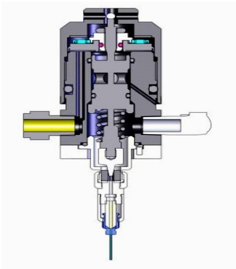
Fig. G18: Sectional drawing of SC-400 jet valve with pulse width modulation
