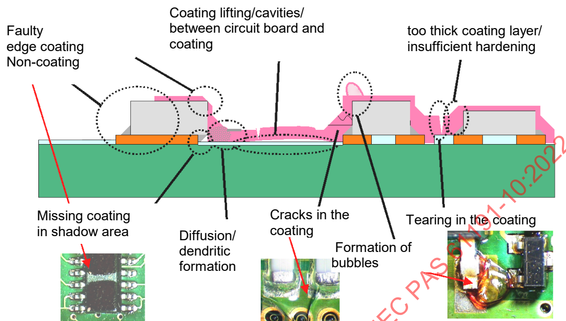
Fig. I1: Incorrect execution of protective coatings
