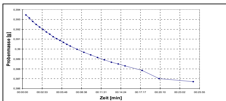
Fig. D3: Time course of the water release of an approx. 60 µm thick PUR coating film (16 h / 80°C cross-linked) in climate 20°C, 55 % rh
