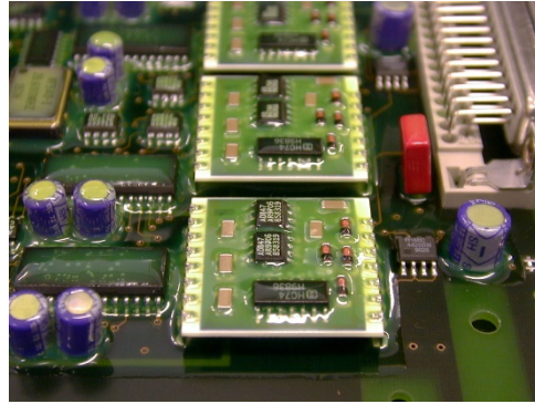
Fig. C22: Examples for a coating with thick-film protective coating
