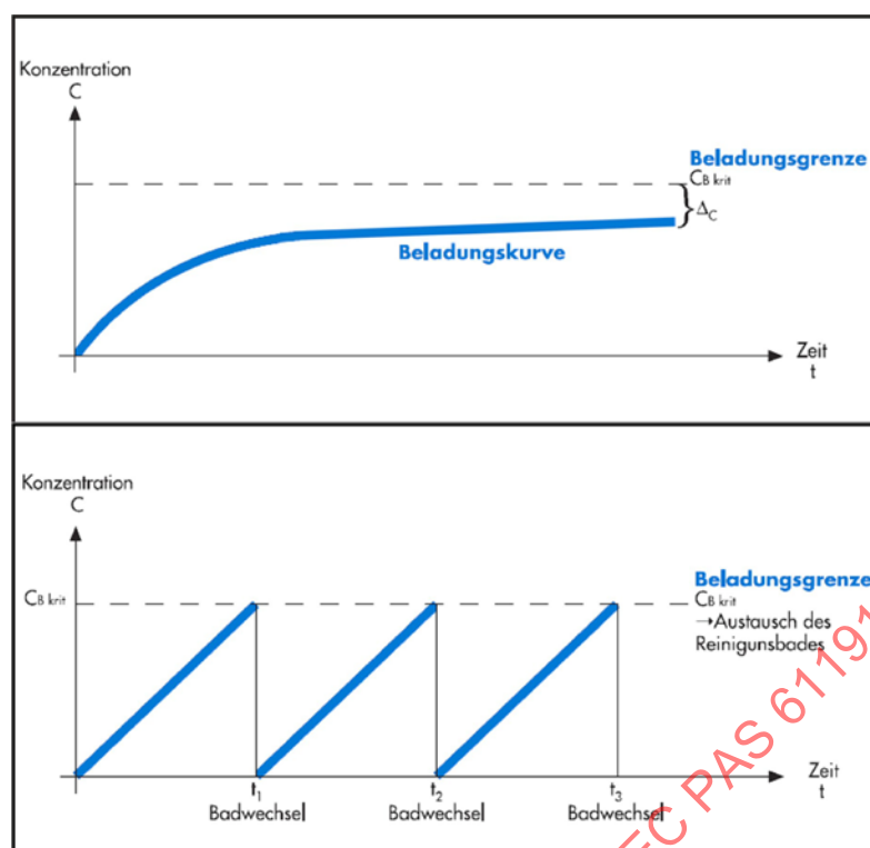
Fig. F8: Comparison of bath service life of surfactant cleaners (bottom) and MPC® cleaners (top)
