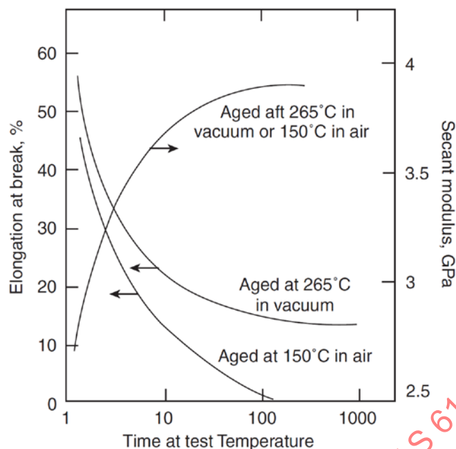
Fig. C13: Effect of temperature on the flexibility of Parylene C in air and vacuum (To convert GPa to psi, multiply by 145,000)
