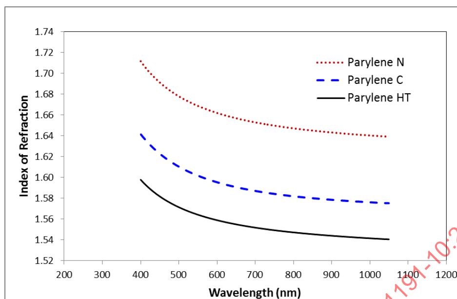
Abb. C21: Parylenes - Index of refraction vs. wavelength (Data courtesy of Filmetrics, Inc)
