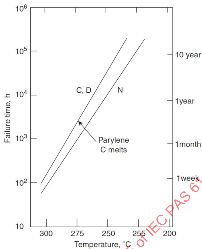
Fig. C14: Long-term effect of aging in vacuum on flexibility of Parylenes at elevated temperature (Failure = 50% loss in tensile strength)
