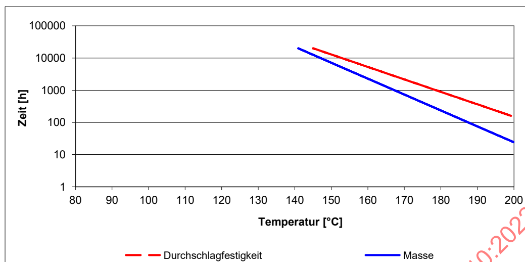
Fig. D10: Extrapolation of the experimentally determined downtimes to a downtime of 20,000 hours (schematic diagram).
