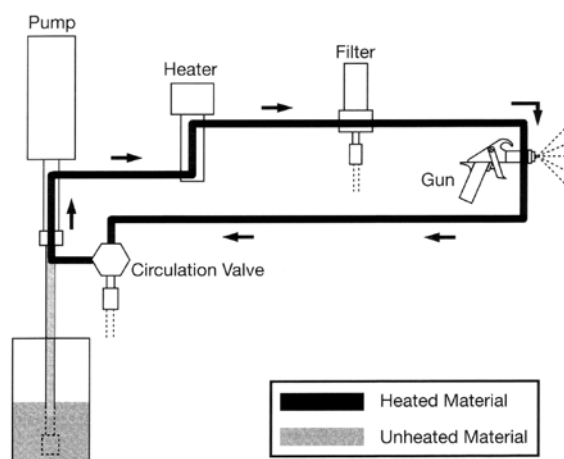
Fig. G15: Closed and recirculating fluid system
