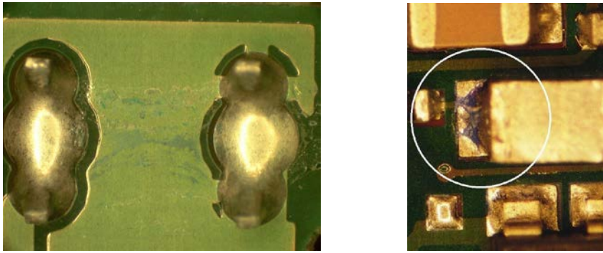
Fig. F5: Creepage current path (left) or flux residues (right) visibly displayed by means of the Zestron® Flux Test
