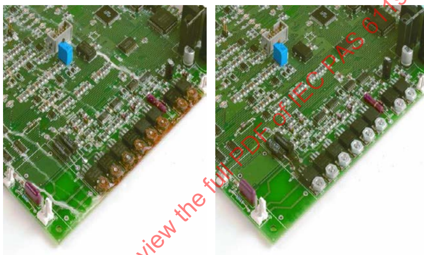
Fig. C15: Uncoated (left) and Parylene HT coated (right) PCB boards after 144 hours salt fog test
