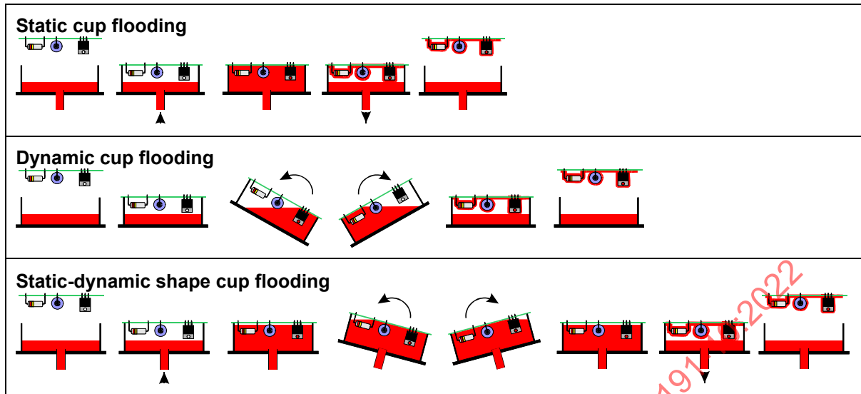
Fig. G5: Schematic representation of the cup flooding process
