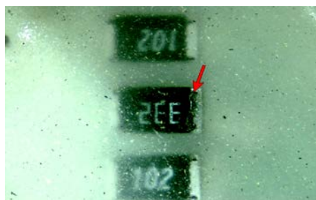
Fig. F1: Example of infiltration of a protective coating compound due to insufficient adhesion due to electrochemical migration
