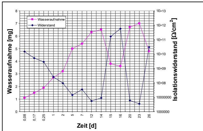
Fig. D1: Time course of the specific resistance as a function of the absorbed water quantity (PUR dip coating cross-linked to FR4, 16 h / 80°C)
