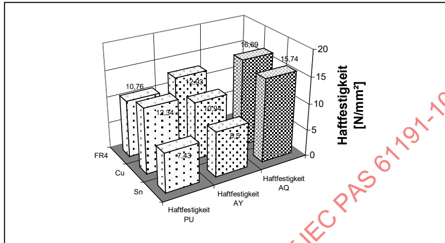
Fig. D6: Adhesion of fully cured samples (4 weeks / 80°C) depending on the type of coating and substrate
