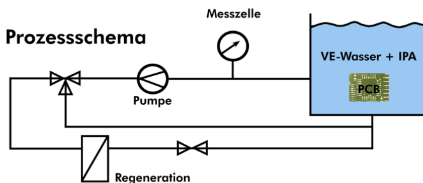
Fig. F3: Scheme for the determination of the ion equivalent by the contaminometer method
