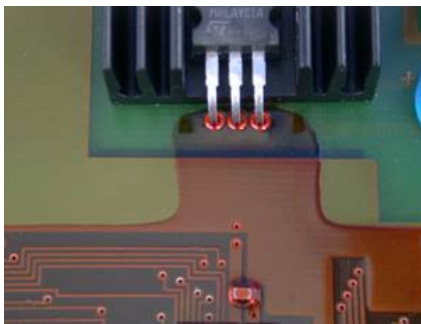
Fig. G11: Power transistor with all-round coated terminals
