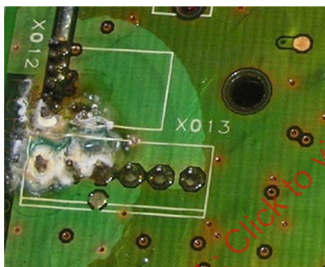
Fig. F2: Delamination and cracking of the protective coating
