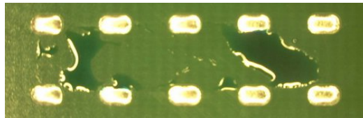
Poor wetting = Impure surface
