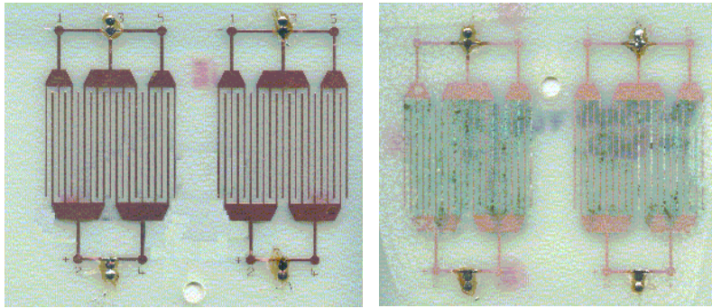
Fig. D11: Exemplary mixture of an acrylic resin coating with a typical solder paste resin under high humidity load (85°C/85 % RH) (left) and condensation (40°C/100 % RH) 10 (Work drawing Lackwerke Peters GmbH + Co KG)
