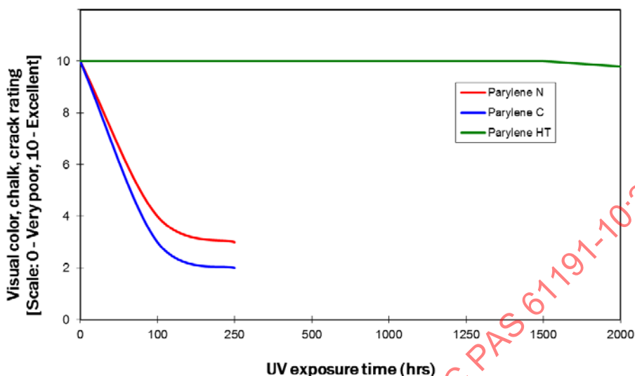
Fig. C20: UV exposure results of Parylene N, C and Parylene HT
