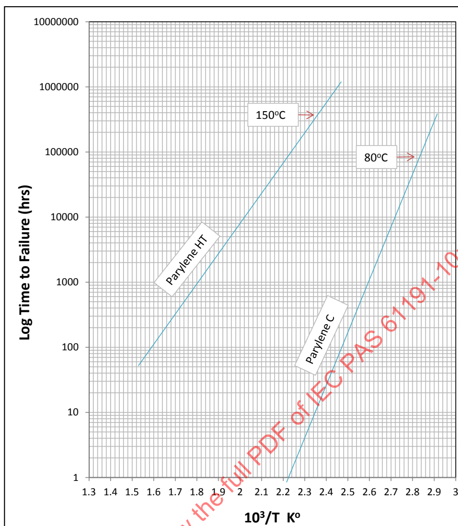
Fig. C12: Useful lifetime of Parylene HT and Parylene C as a function of temperature in air
