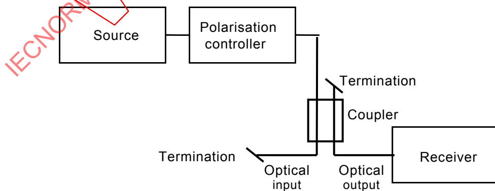
Figure A3 – Set-up for measurement of system constant
