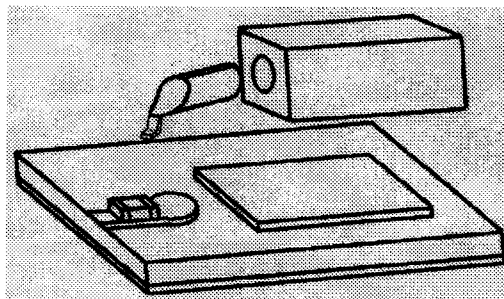
Figure 5.6. Rectangular type \lambda/4 TEM mode resonator mounted on PWB.
