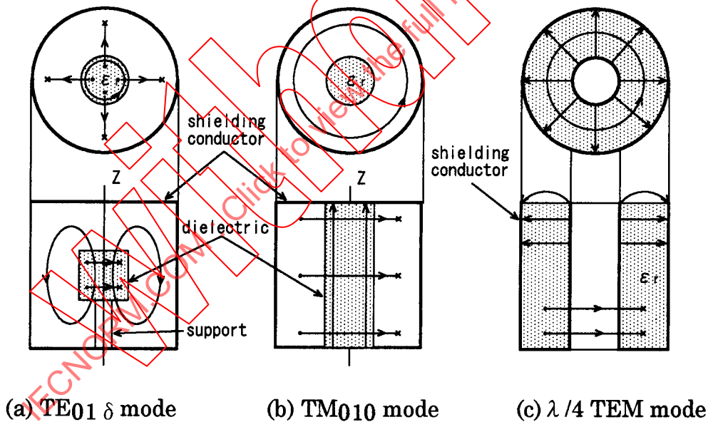
Figure 4.2 TE 01δ mode, TM 010 mode, and Quarter wavelength TEM mode dielectric resonators.
