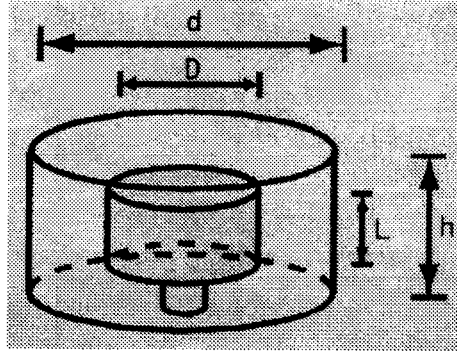
Figure 5.3. Dimension of TE 01δ mode resonator.
