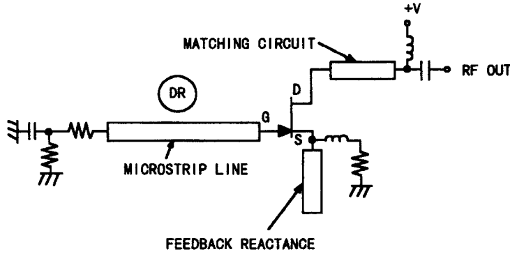
Fig. 6.2 Example of reflection type oscillator.
