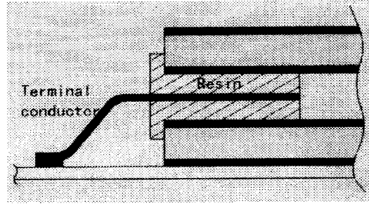
Figure 5.7. TEM mode resonator with metal terminal molded by resin.
