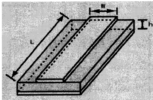
Figure 5.10. Microstripline resonator.
