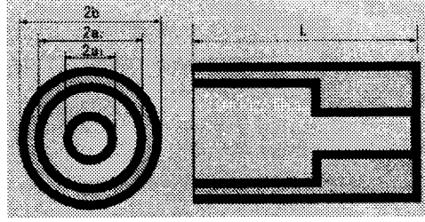
Figure 5.9. \lambda/4 TEM mode resonators with stepped inner diameter.
