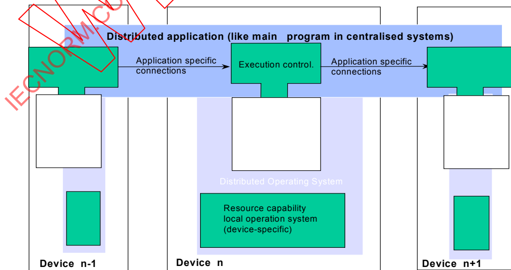
Figure C.4 – Distributed application and distributed operating system
