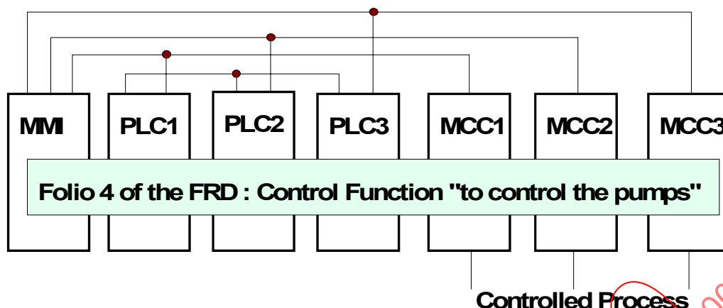
Figure A.27 – Distribution of the control function "to control the pumps" using the IEC 61499-1
