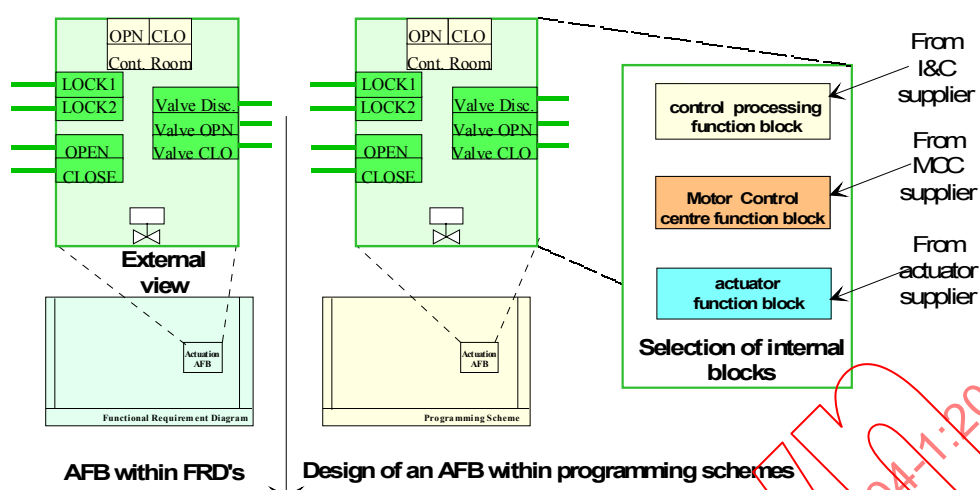
Figure A.16 – Designing internal behaviour of actuation AB from actuation devices of the shelf
