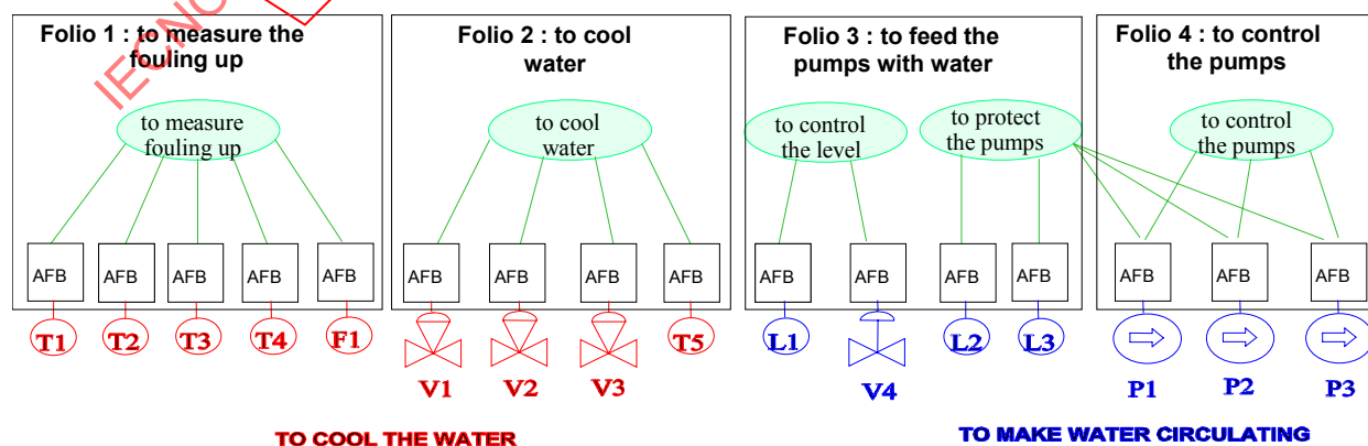
Figure A.6 – Structured documentation for the requirements of the control functions
