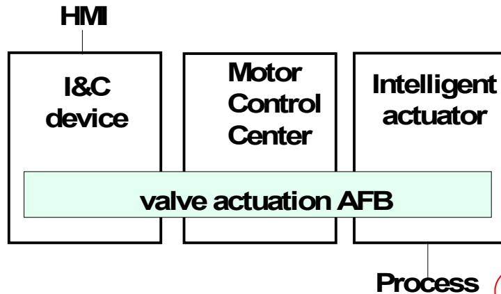
Figure A.19 – OFF/ON value actuation AB using the IEC 61499-1 system model
