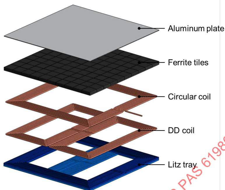
Figure B.7 – General layout of the MF-WPT4/Z3 reference secondary device
