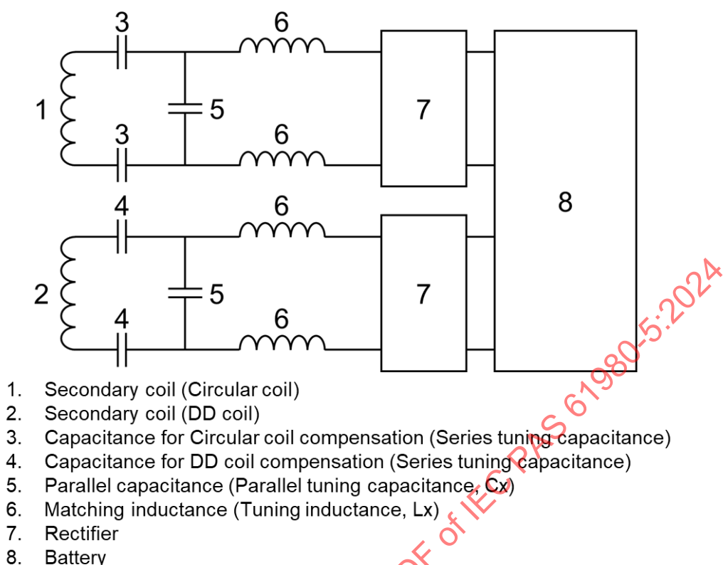
Figure B.3 – Schematic of the EV power electronics for the MF-WPT4/Z1 reference EVPC
