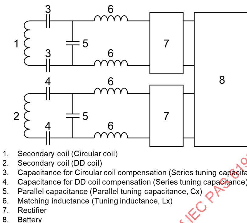
Figure B.12 – Schematic of the EV power electronics for the MF-WPT5/Z1 reference EVPC
