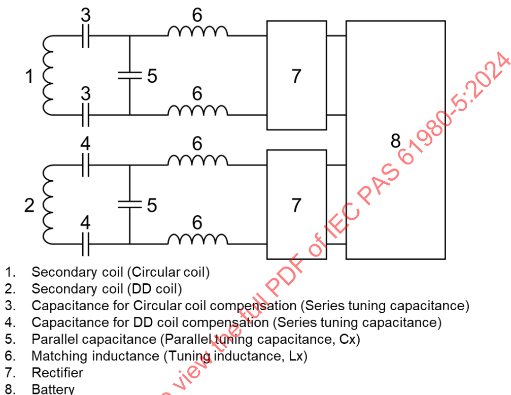
Figure B.15 – Schematic of the EV power electronics for the MF-WPT5/Z2 reference EVPC
