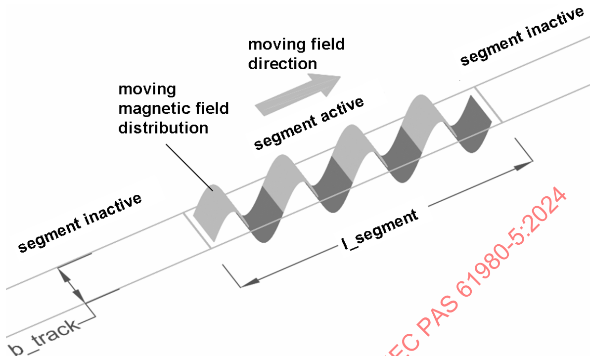
Figure C.2 – Magnetic field distribution of reference primary coil device
