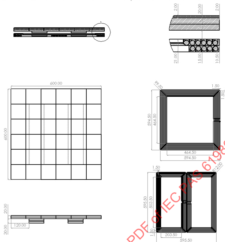
Figure B.17 – Mechanical dimensions of the MF-WPT5/Z3 reference secondary device
