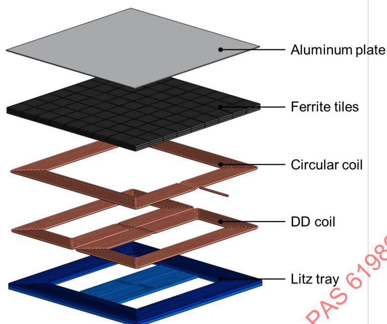
Figure B.4 – General layout of the MF-WPT4/Z2 reference secondary device
