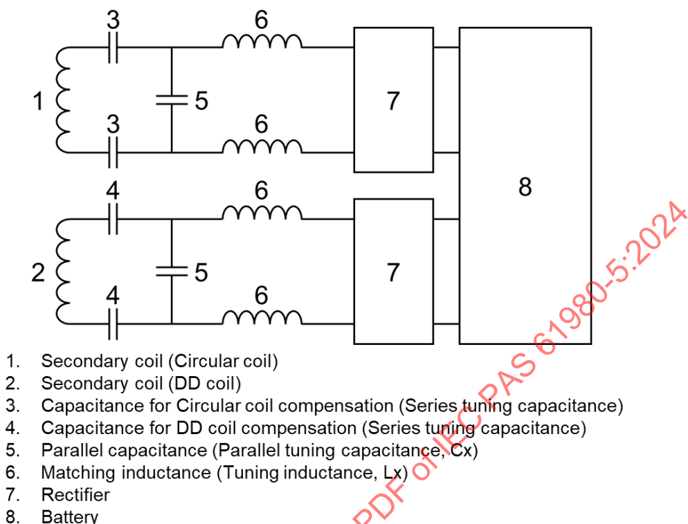
Figure B.6 – Schematic of the EV power electronics for the MF-WPT4/Z2 reference EVPC
