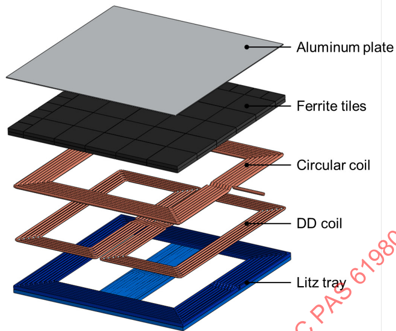
Figure B.13 – General layout of the MF-WPT5/Z2 reference secondary device
