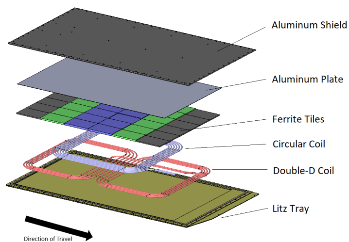
Figure A.16 – General layout of the MF-WPT5/Z3 reference secondary device
