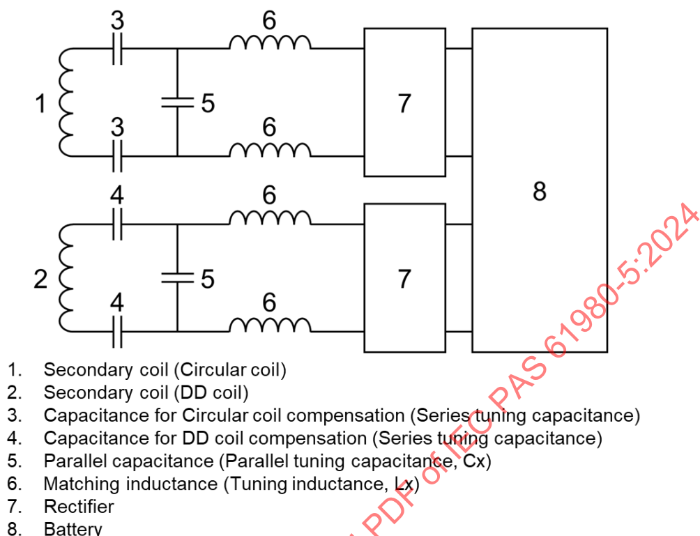
Figure B.9 – Schematic of the EV power electronics for the MF-WPT4/Z3 reference EVPC
