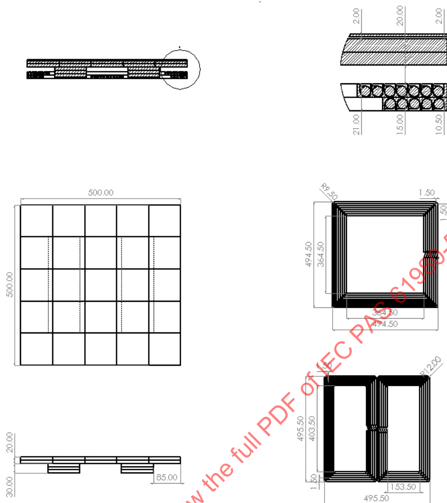
Figure B.11 – Mechanical dimensions of the MF-WPT5/Z1 reference secondary device
