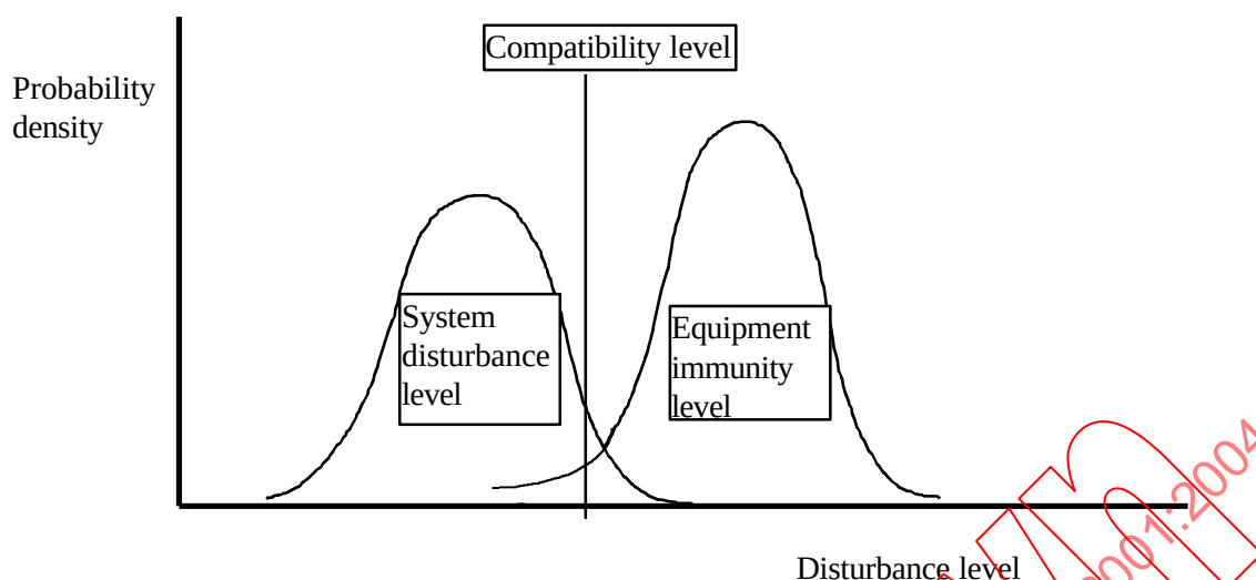
Figure 7.9 Illustration of basic voltage quality concepts with time/location statistics covering the whole system (adapted from [Ref. 7-11])
