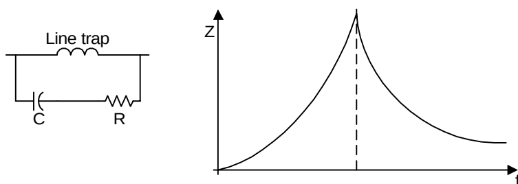
Figure 12-2 Single-tuned series filter and impedance plot
