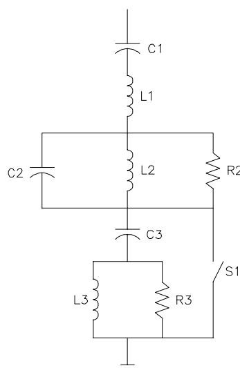
Figure 12.5 Re-tunable a.c. filter branch
