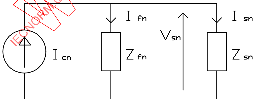
Figure 7.1 Circuit model for filter calculations
