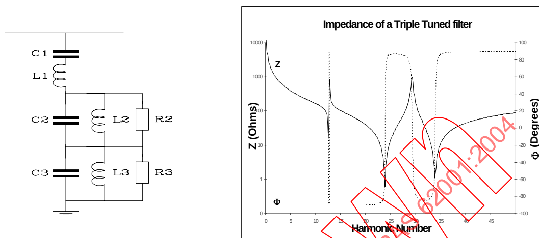
Figure 6.3 Triple tuned filter and frequency response
