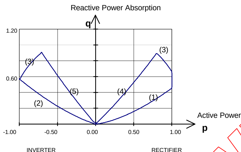
Figure A8.2 Converter capability with \gamma_{\min}=17^\circ , \gamma_{\max}=40^\circ , \alpha_{\min}=5^\circ , \alpha_{\max}=35^\circ and U_{\text{diomax}}=1.2U_{\text{dioN}}
