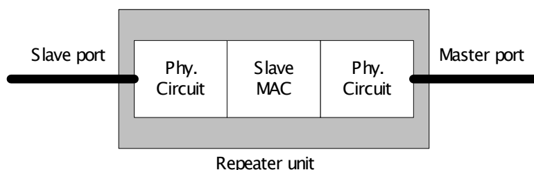
Figure 56 – Repeater MAC and Phy. circuit diagram
