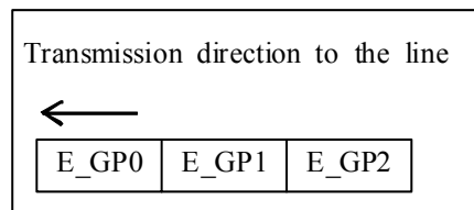
Figure 23 – Group block
