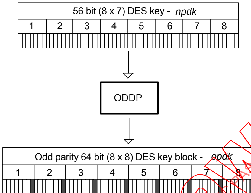
Figure 2 – Odd parity function ODDP
