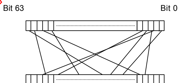
Figure 8 — Illustration of the permutation process used for decryption
