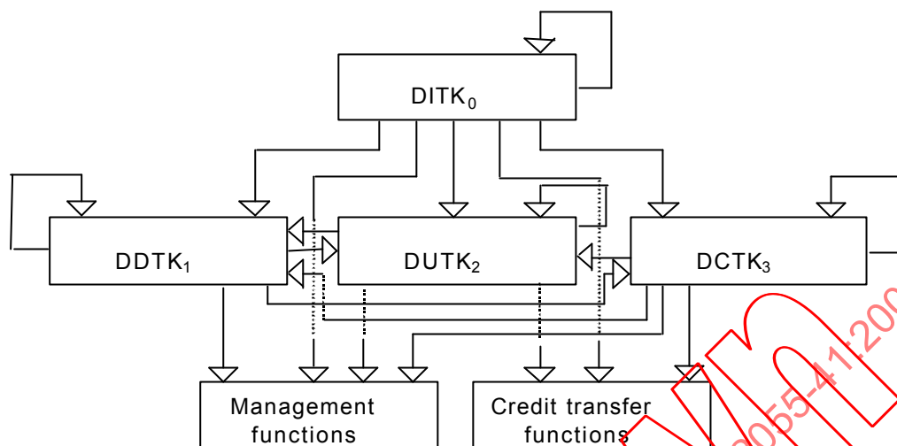
Figure 1 – Relationships among STS key types
