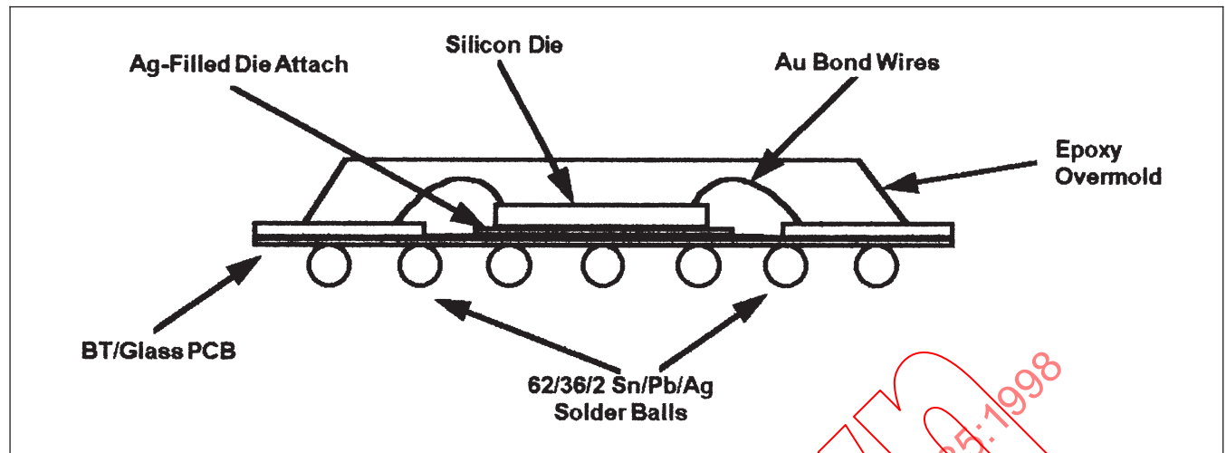
Figure 4-8 Plastic BGA Cross Section
