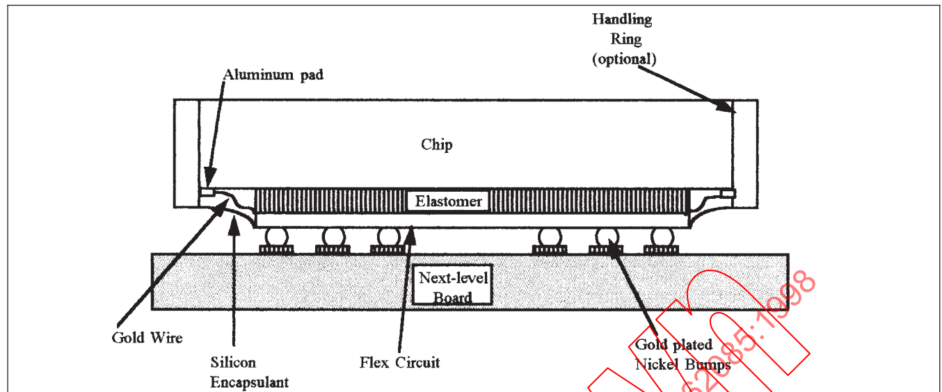
Figure 4-12 Micro BGA
