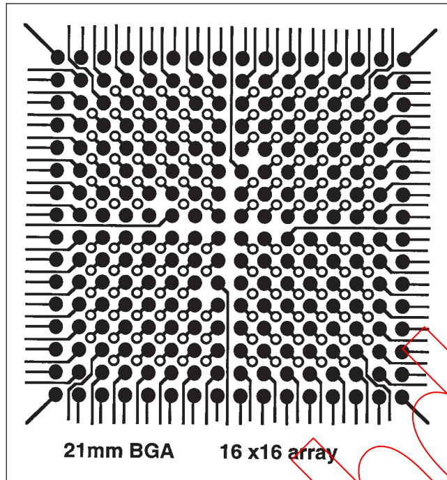
Figure 5-4 PWB Top Surface Including Vias
