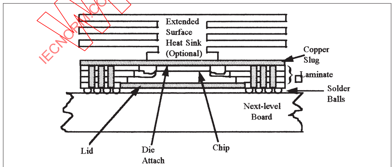
Figure 4-9 Thermally Enhanced BGA
