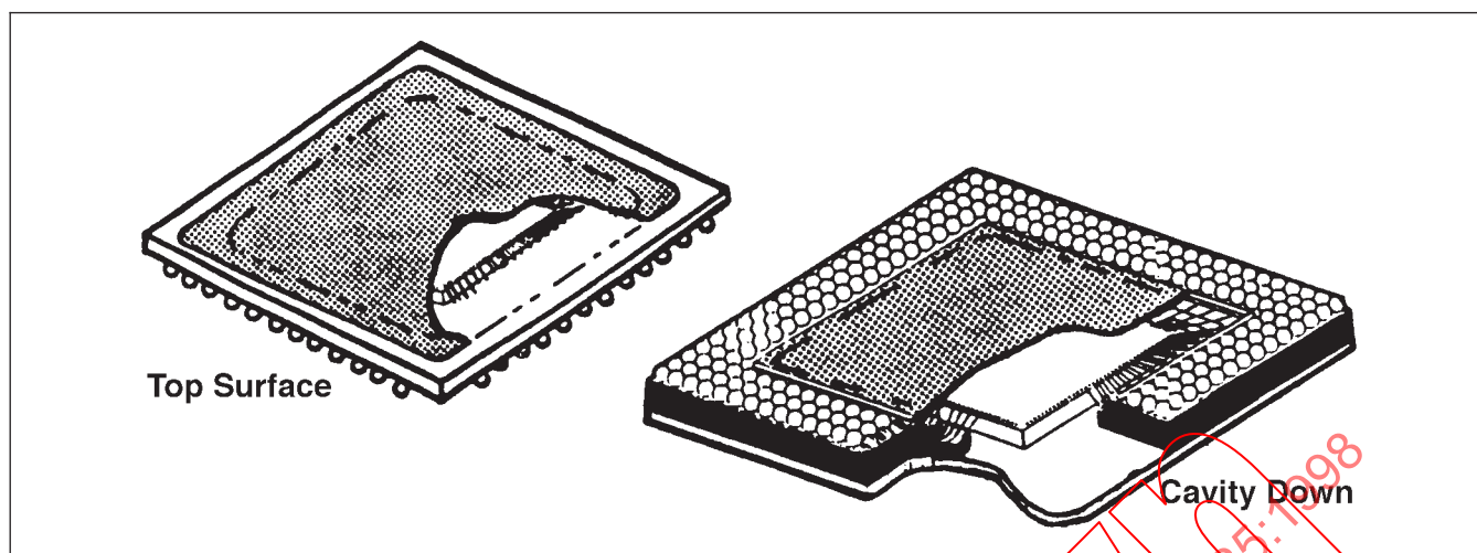
Figure 4-1 Ball Grid Array Devices Furnished with Die Mounted on Top Surface and Bottom Side for Cavity Down
