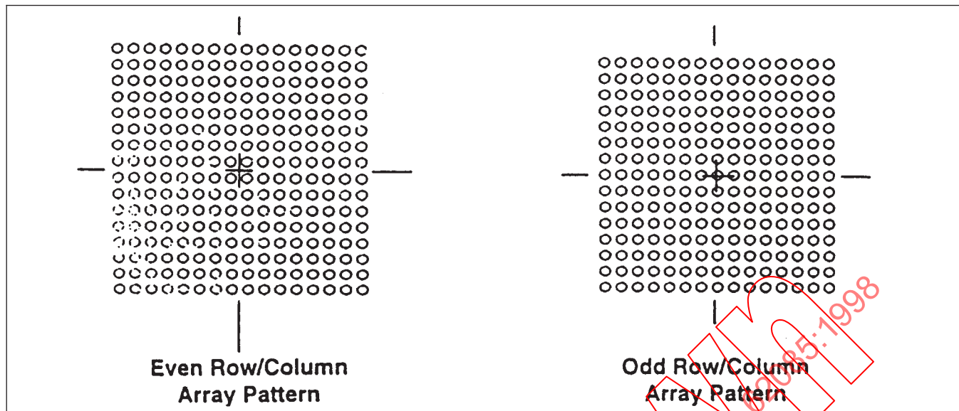
Figure 4-15 Both Even and Odd Column and Row Patterns Are Permitted in the JEDEC Standards
