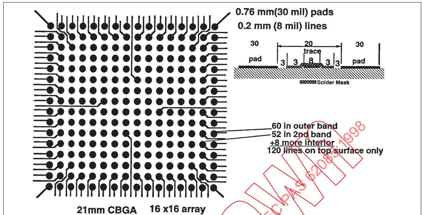
Figure 5-5 First Two Rows of the Array Escape on the Top Surface
