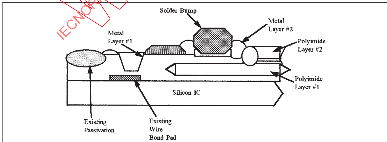
Figure 4-11 On-Chip Pad Redistribution (Sandia Mini BGA)
