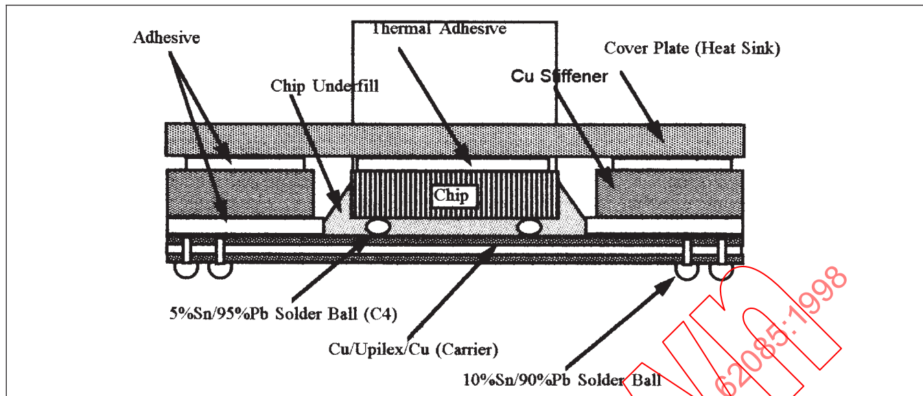
Figure 4-10 Cross-Section of a TBGA Package
