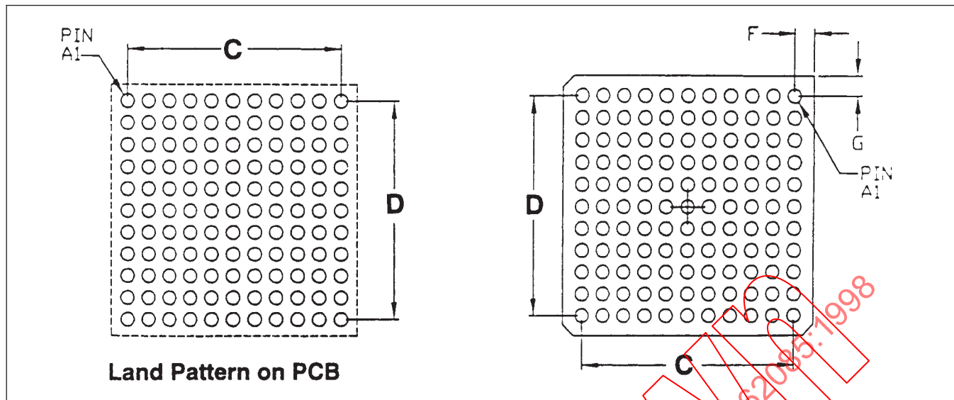
Figure 4-5 Contact Patterns
