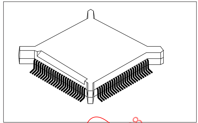
Figure 4-18 FQFP Construction
