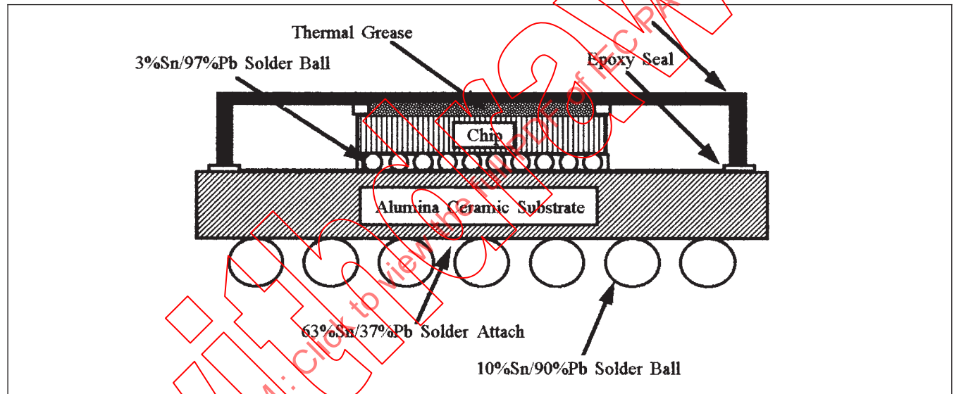
Figure 4-13 Cross-Section of CBGA
