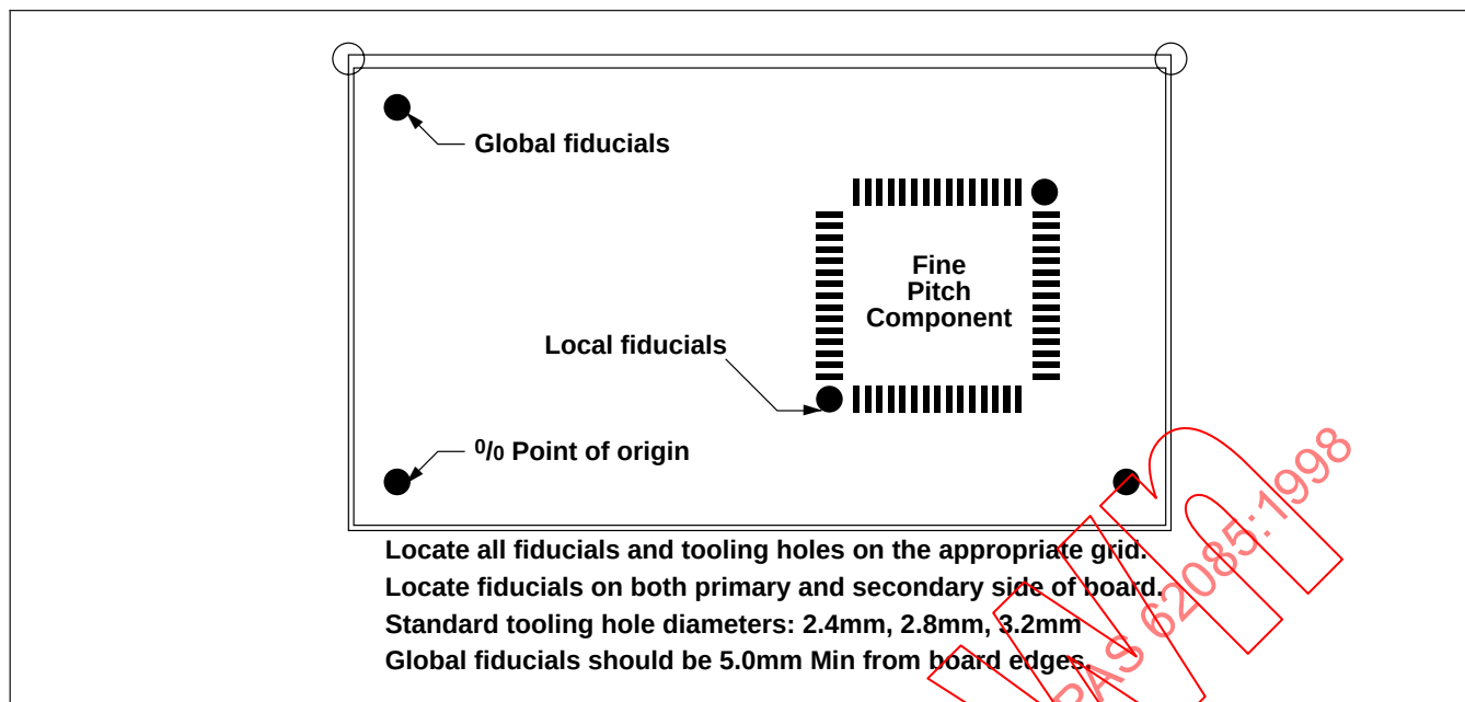
Figure 6-5 Fiducial Locations on a Printed Circuit Board
