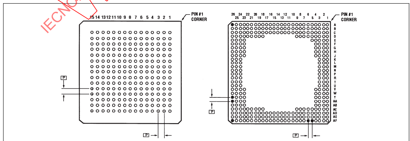
Figure 4-14 BGA Devices Having the Same Physical Size and I/O Count
