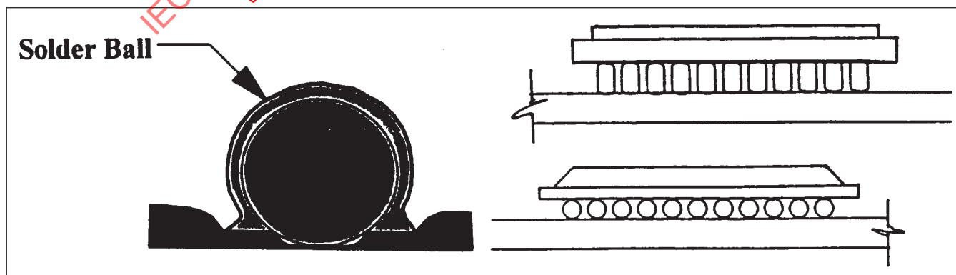
Figure 4-2 Stand Off Height
