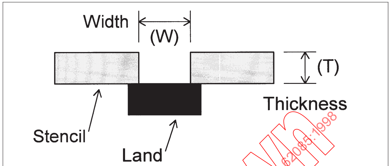
Figure 6-3 Stencil Opening Aspect Ratio
