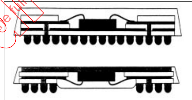
Figure 4-7 Cavity-up and Cavity-down Chip Mounting
