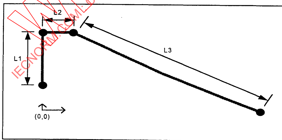
Figure 6 — Bond wire sections for simplified model
