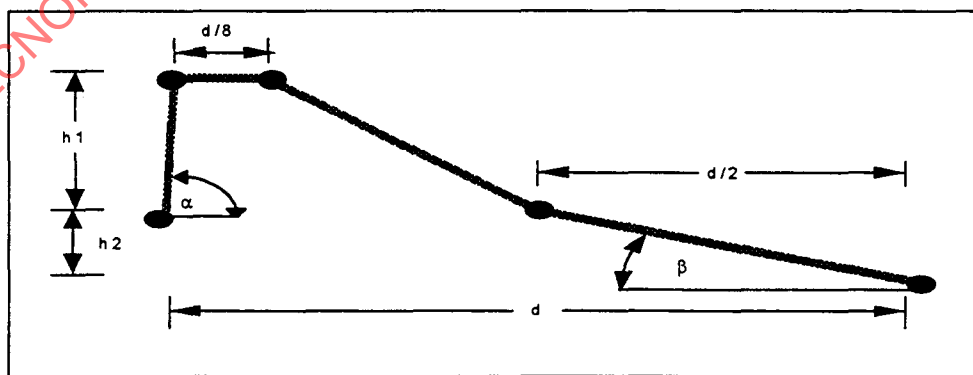
Figure 1 — Parameters and constraints
