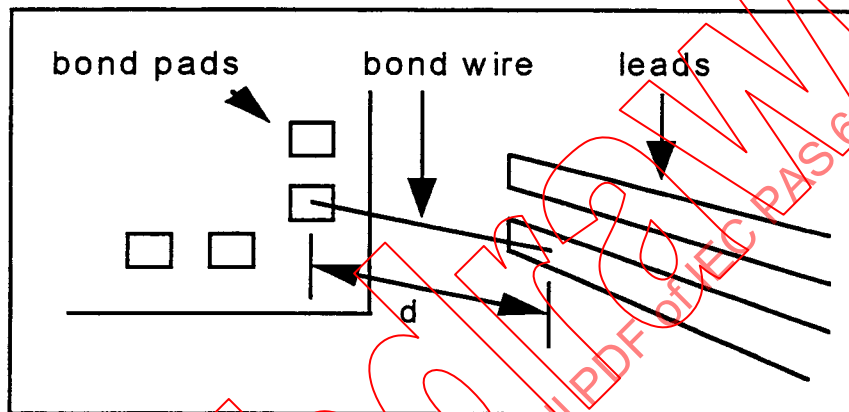
Figure 7—Top view of bond wire
