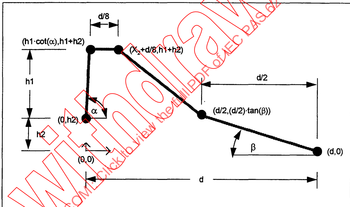
Figure 3 — Parameters and coordinates
