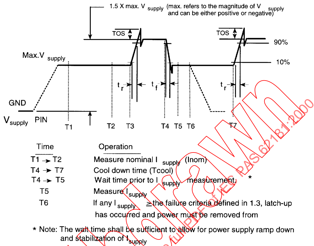
Figure 4 — Test waveform for V_{supply} overvoltage
