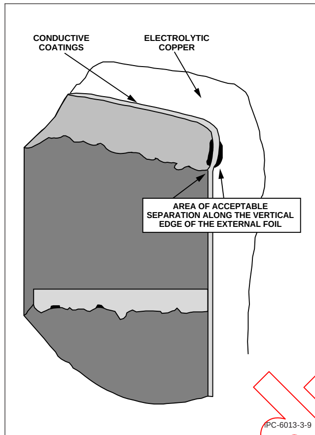
Figure 3-9 Separation at External Foil
