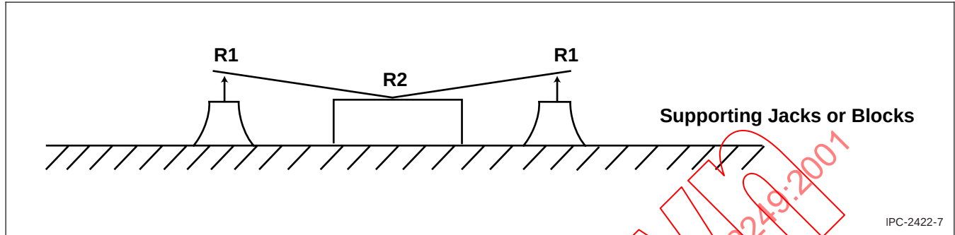
Figure 7 Corners Supports
