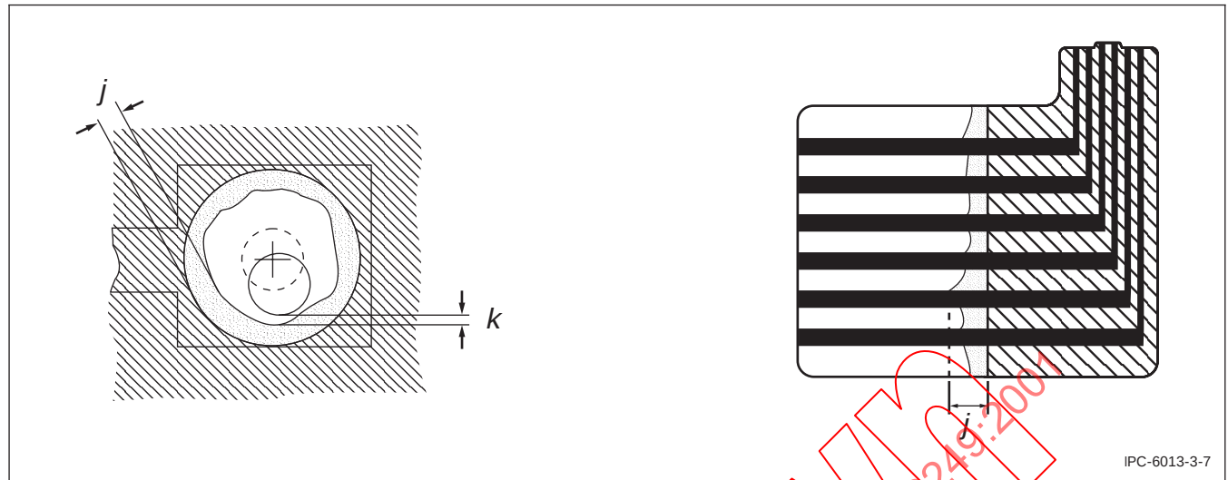
Figure 3-7 Squeeze-Out of Coverlay and Ooze-Out of Covercoat
