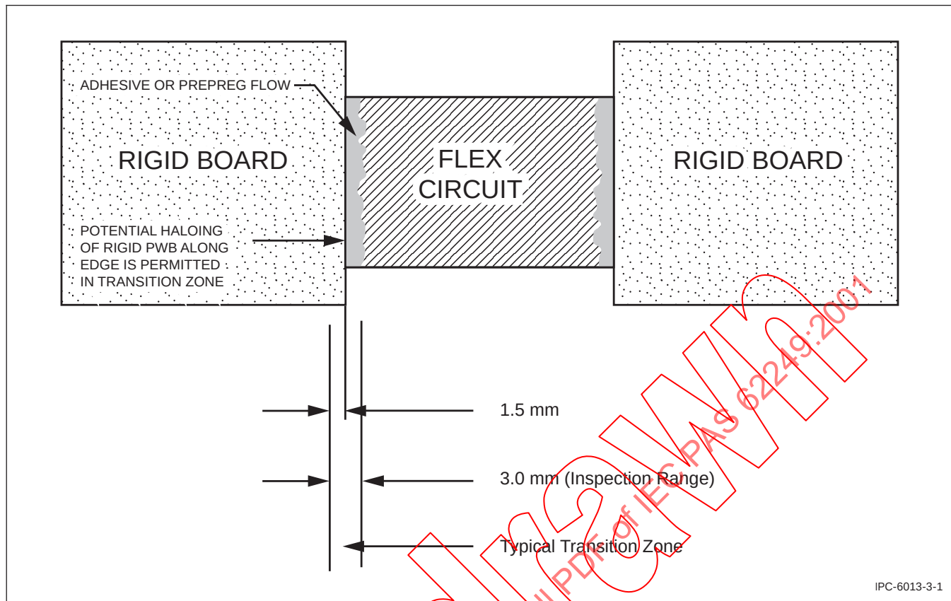
Figure 3-1 Transition Zone
