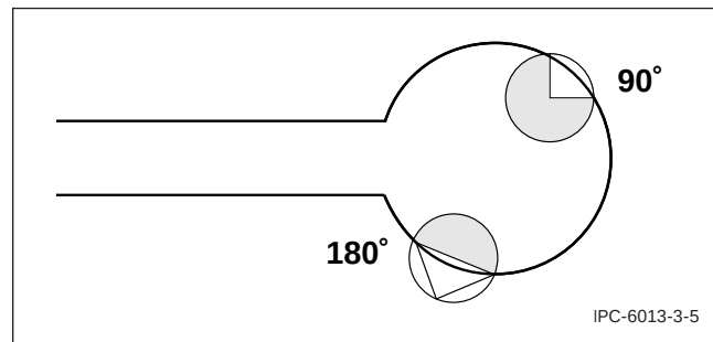
Figure 3-5 Breakout of 90° and 180°
