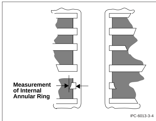
Figure 3-4 Annular Ring Measurement
