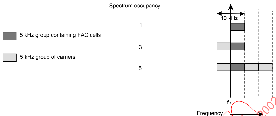
Figure 29: Spectrum occupancy for 10 kHz channels
