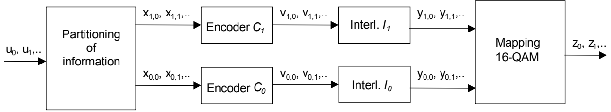
Figure 20: Multilevel coding with 2 levels (SM)
