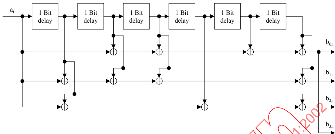
Figure 22: Convolutional encoder
