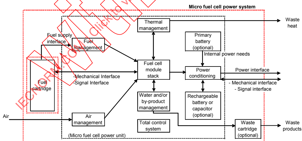
Figure A.1 – Formic acid fuel cell system diagram
