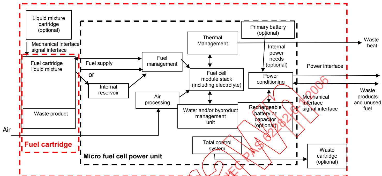
Figure E.1 – Direct borohydride fuel cell power unit
