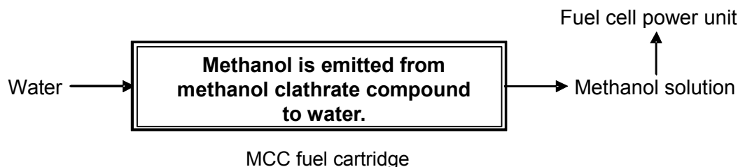
Figure D.3 – Usage of methanol clathrate compound with fuel cell power unit.
