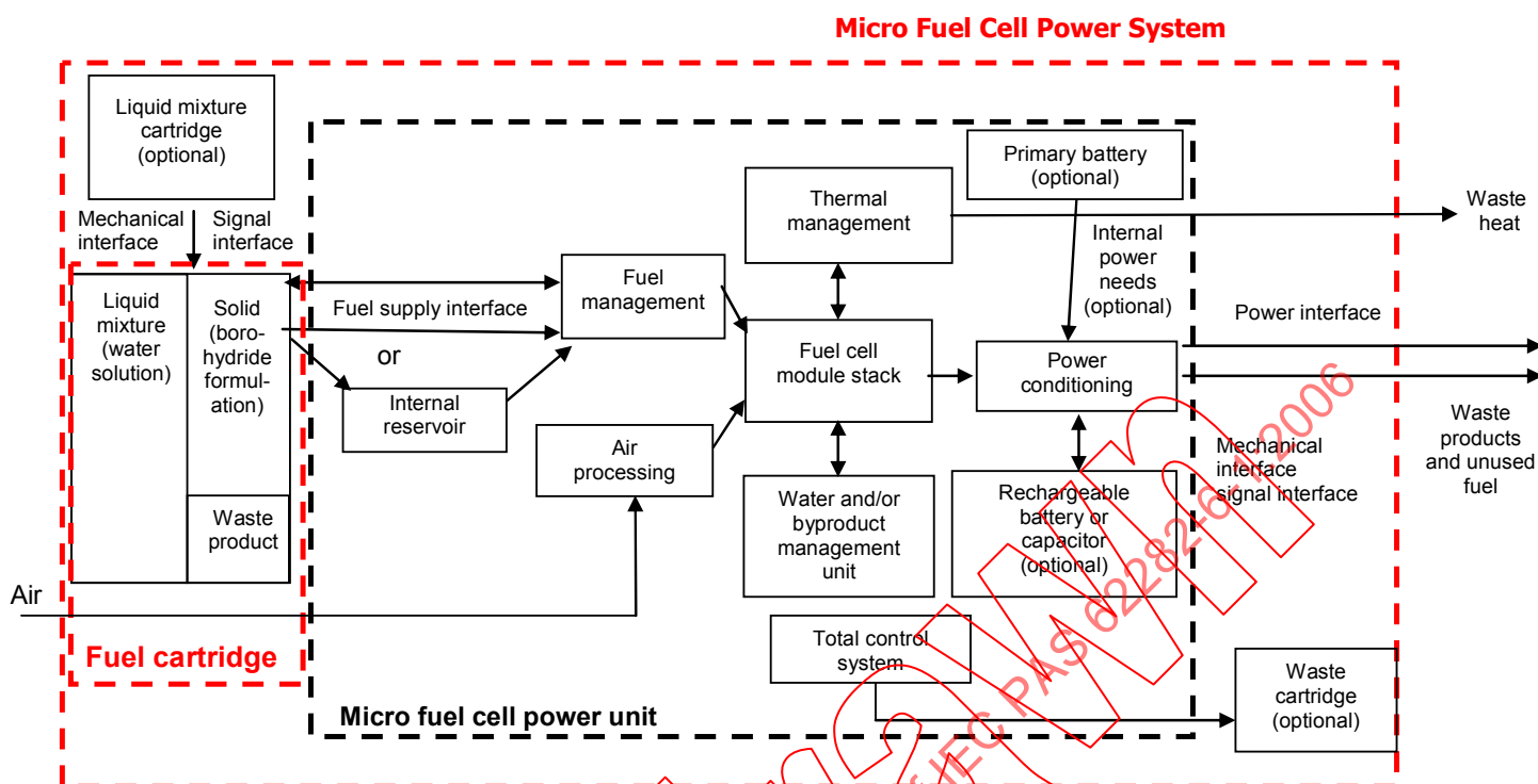
Figure E.2 – Indirect borohydride fuel cell power unit
