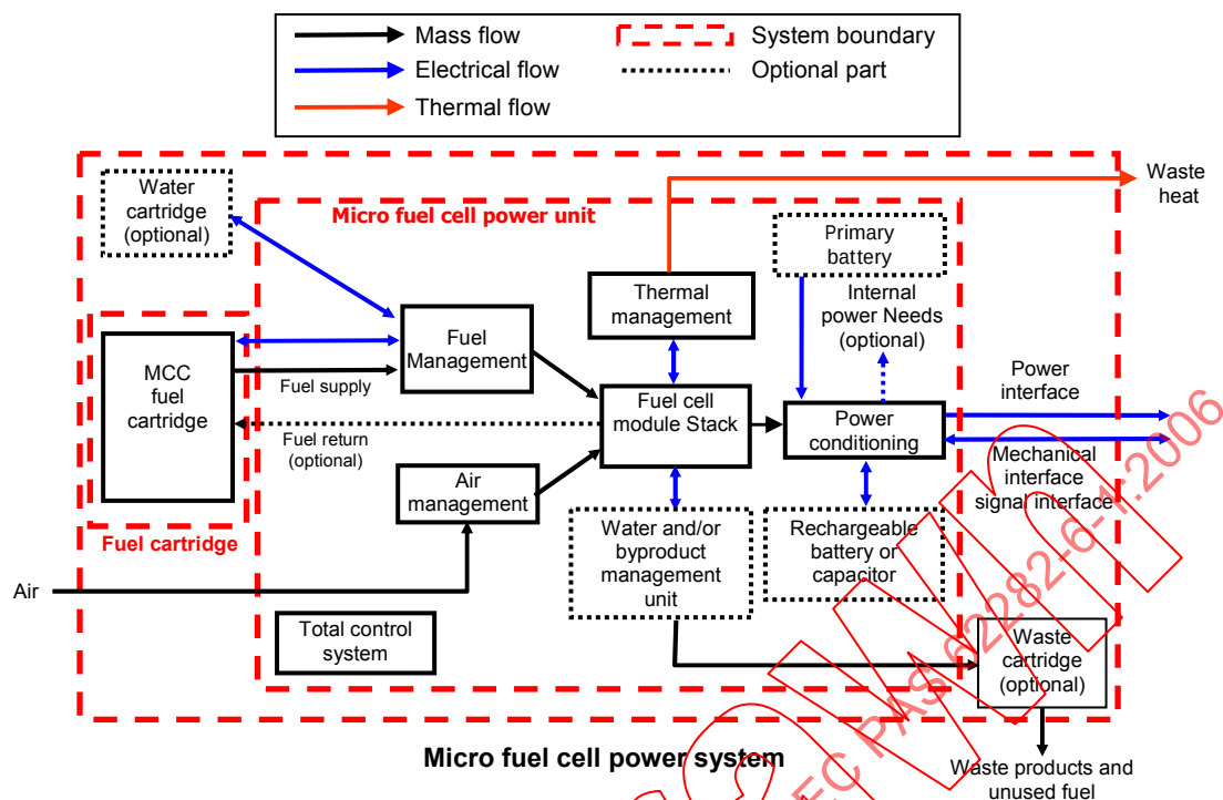
Figure D.1 – General block diagram of direct methanol fuel cells powered by methanol clathrate compound
