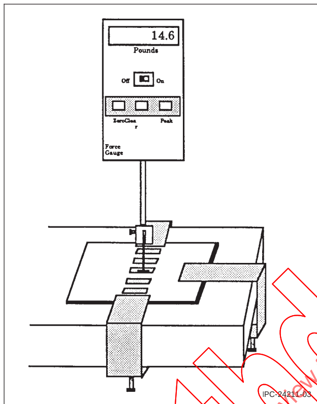
Figure 3 Pull Tester
