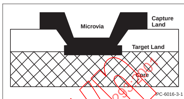
Figure 3-1 Typical Microvia Structure
