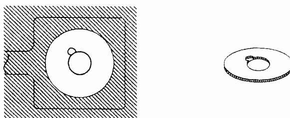
Figure 3 – Circumferential void at the component hole
