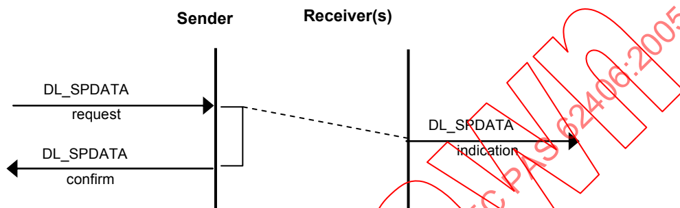
Figure 7 – Sequence diagram of Sporadic Message service
