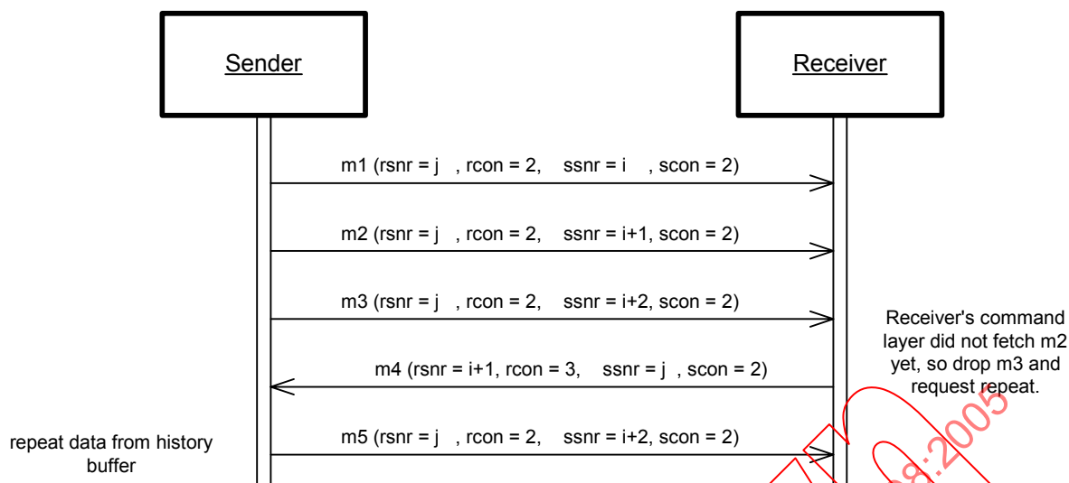
Figure 47 – Error Flooding with asynchronous commands
