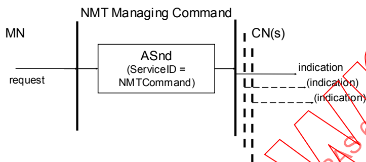
Figure 72 – NMT Managing Command Service Protocol
