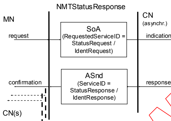
Figure 74 – NMT Response Service Protocol (Acyclic-only CN)
