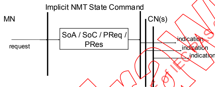
Figure 70 – Implicit NMT State Command Service Protocol
