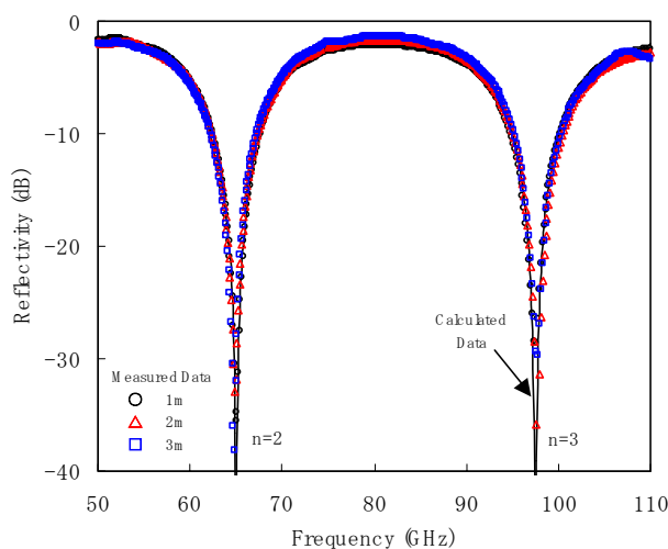
Figure B.2 – Reflectivity of a 75mm × 75 mm sapphire crystal (001) plate in millimetre wave frequency
