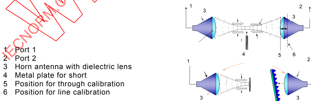
Figure D.2 – Measurement and TRL calibration of transmission line
