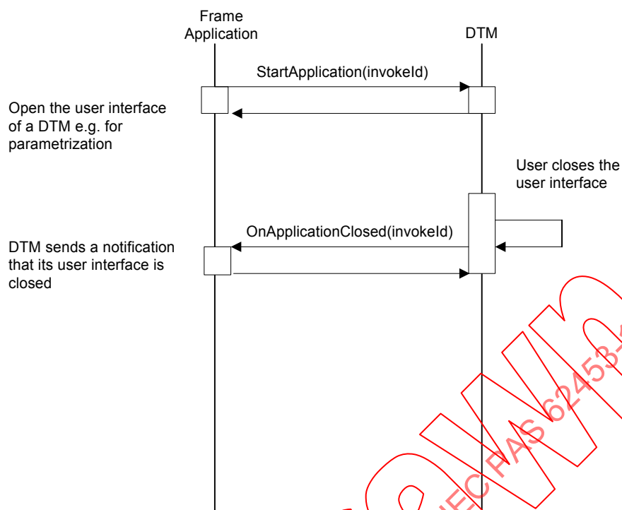
Figure 68 – Starting and releasing applications
