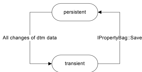
Figure 84 – Persistence states of a data set
