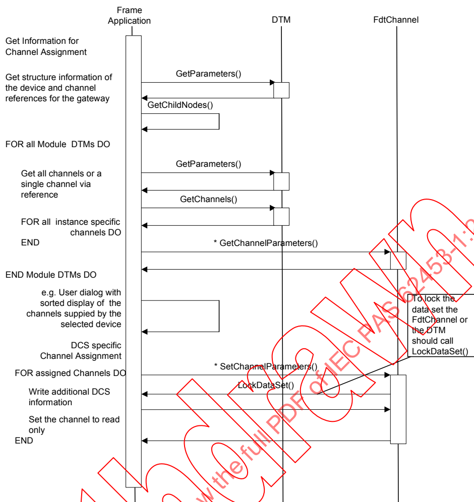
Figure 73 – Channel assignment for modular DTM
