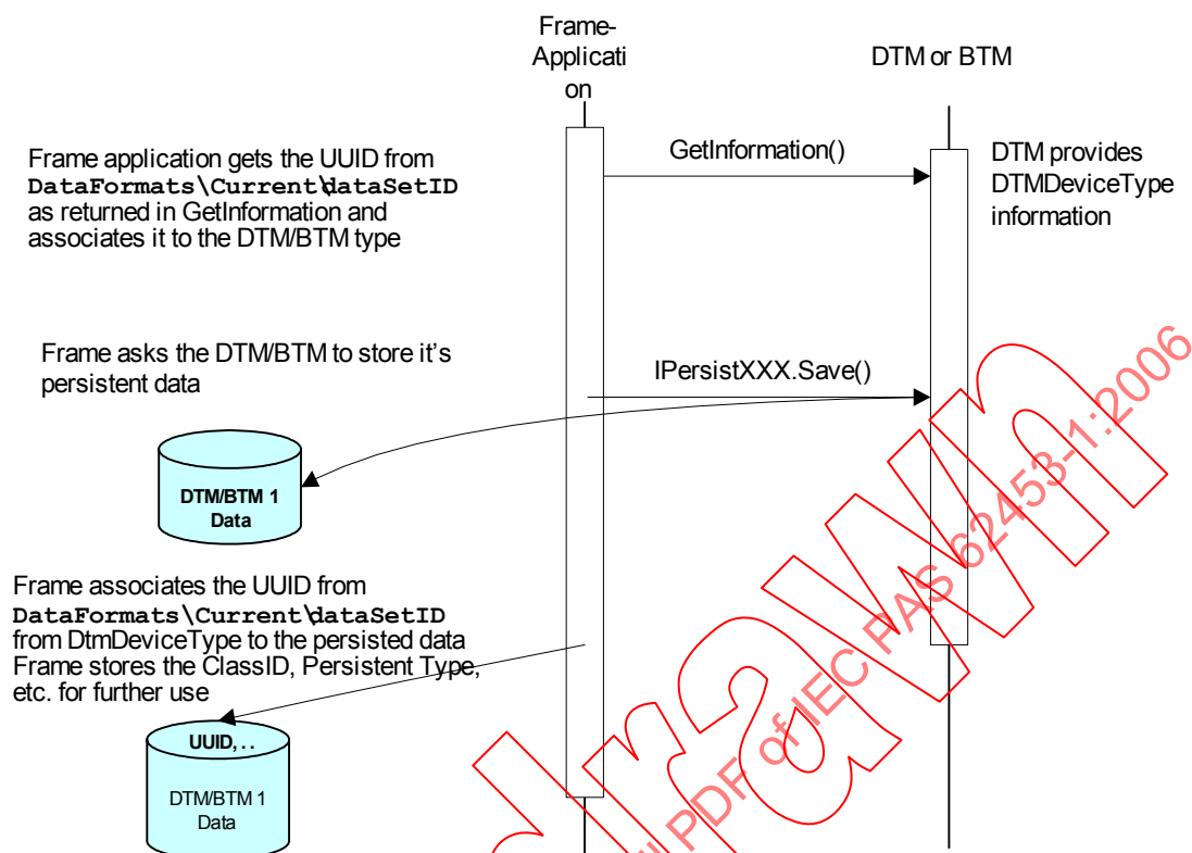
Figure 99 – Saving data from a DTM to be upgraded
