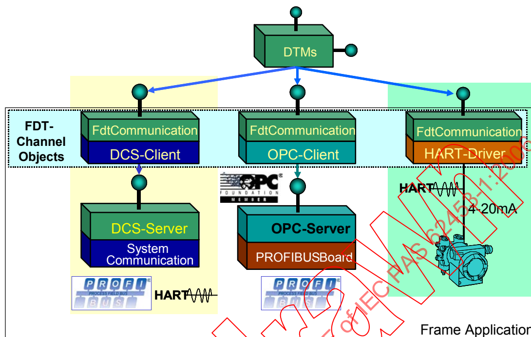
Figure 10 – The FDT communication layers
