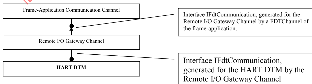
Figure 58 – System connection (across communication hierarchy)
