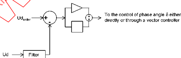
Figure 7.6 - DC voltage-controller
