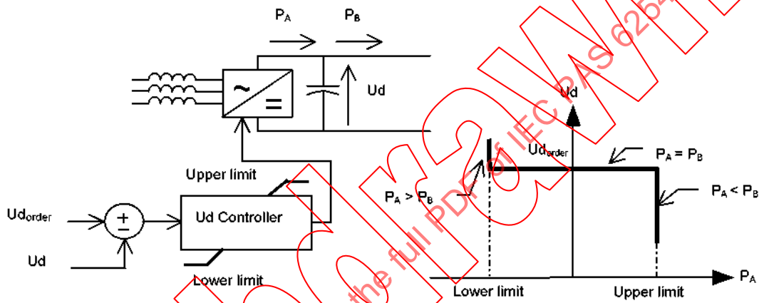
Figure 7.8 - DC voltage control and the U_d - P_d characteristic
