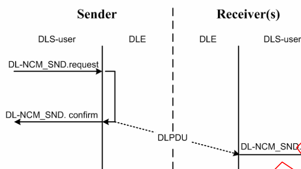
Figure 15 – Sequence diagram of NCM service primitive
