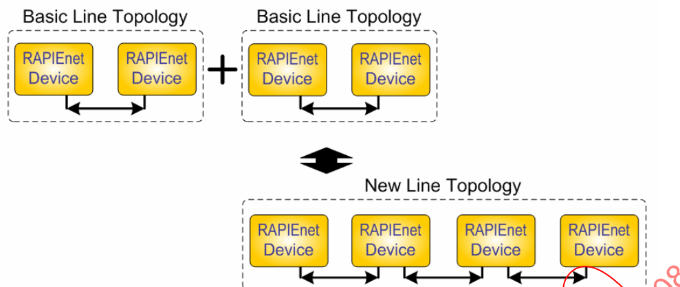
Figure 5 – Line topology
