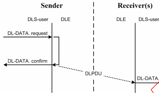
Figure 13 – Sequence diagram of DL-DATA service
