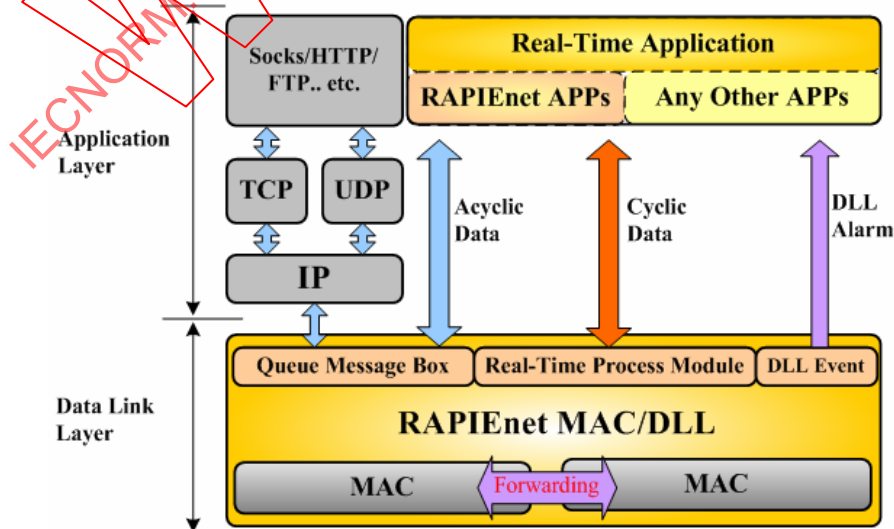
Figure 8 – Interaction between FAL and DLL
