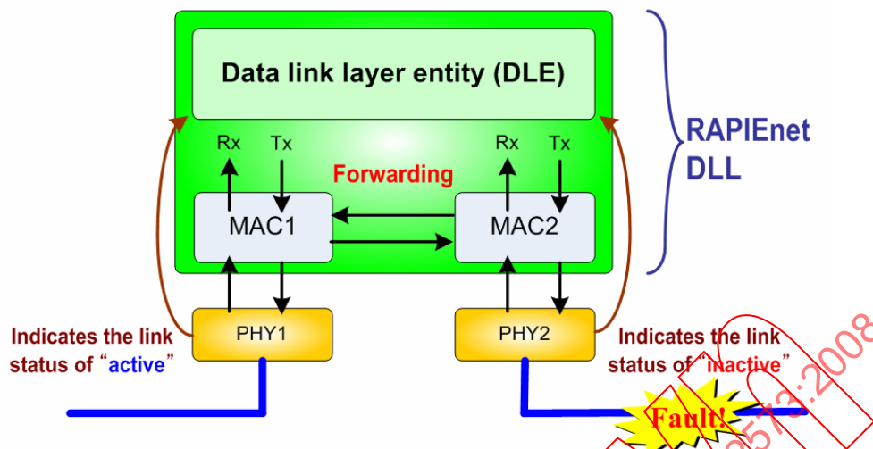
Figure 4 – Link status information
