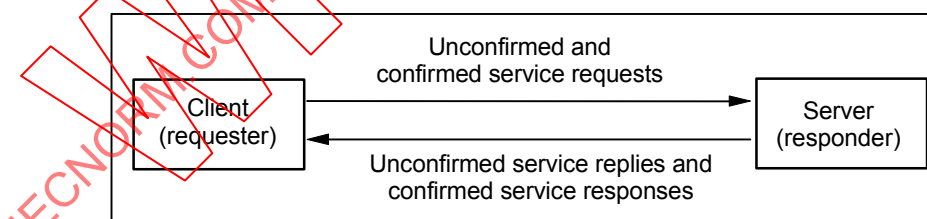
Figure 45 – Client/server interactions
