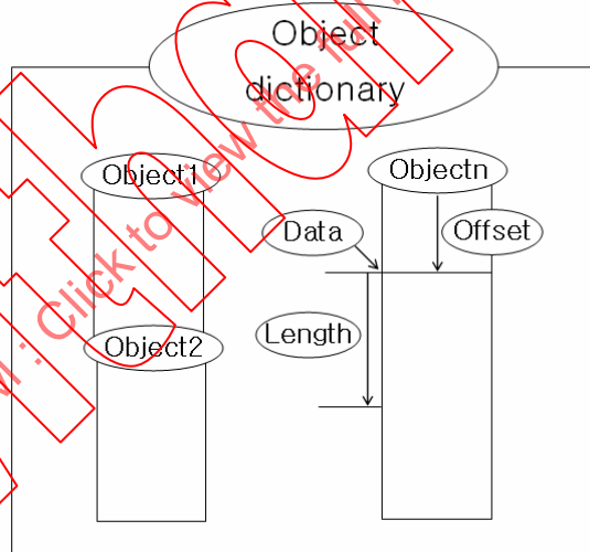
Figure 57 – Object model
