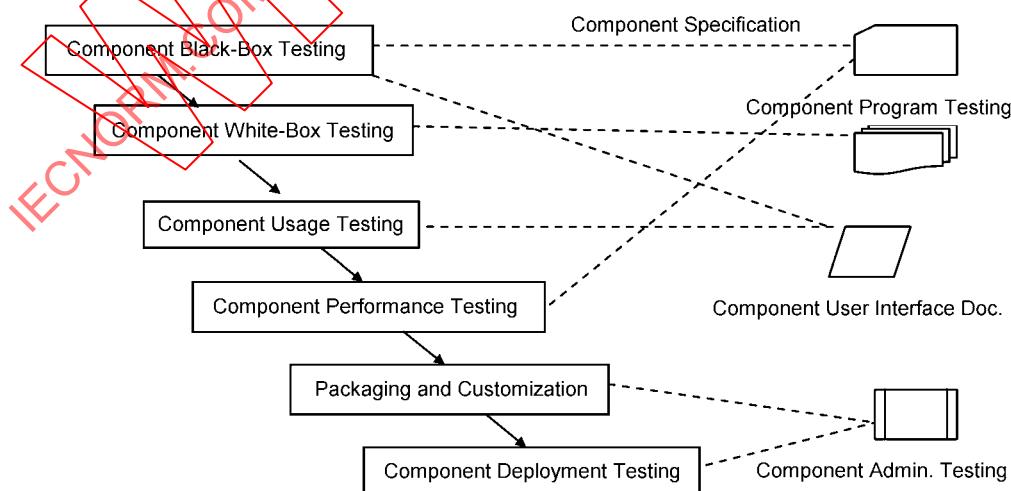
Figure C.1 – A test process in vendor-oriented component testing [30]
