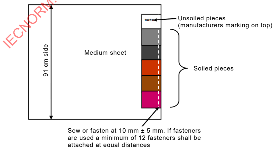
Figure 2 – Attached test strip
